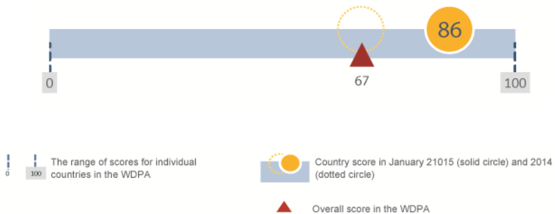
Figure 3.3. Quality indicators for the WDPA monthly release
