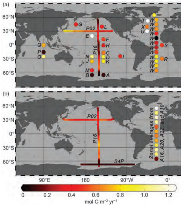
FIG. 3.30. Regional C_{anth} (anthropogenic carbon) storage rate estimates in literature as colored dots with positions corresponding to the approximate centers of the broad regions considered. Estimates are from: A. Williams et al. (2015), B. Sabine et al. (2008), C. Sabine et al. (2008), D. Peng et al. (2003), E. Peng et al. (2003), F. Murata et al. (2009), G. Wakita et al. (2010), H. Sabine et al. (2008), I. Waters et al. (2011), J. Waters et al. (2011), K. Waters et al. (2011), L. Sabine et al. (2008), M. Matear and McNeil (2003), N. Murata et al. (2007), O. Murata et al. (2010), P. Peng et al. (1998), Q. Peng et al. (1998), R. Murata et al. (2008), S. Peng and Wanninkhof (2010), T. Friis et al. (2005), U. Tanhua et al. (2007), V. Olsen et al. (2006), W. Wanninkhof et al. (2010), and X. Quay et al. (2007). Storage rate estimates that use data from cruises in the year 2011 or afterward are mapped in (b), and all other estimates are mapped in (a). Atlantic estimates in (b) are from Woosley et al. (2016). Colored lines are provided representing preliminary storage rate estimates along the labeled P16 and P02 sections in the decades spanning the (a) 1990s to 2000s and (b) 2000s to 2010s occupations. The similar line in (b) for S4P is from Williams et al. (2015).
