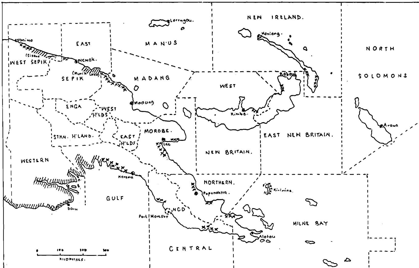
Figure 1. Predicted degree of inundation from anticipated sea level rise.
