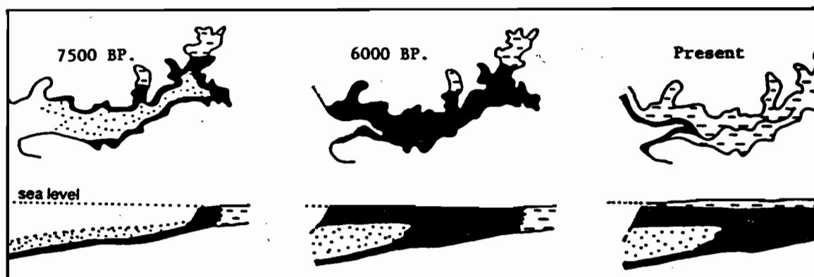
Figure 4. Evolution of the South Alligator plains. When sea level was rising rapidly, 7,500 years ago, the valley was a broad shallow estuary fringed with mangrove. As sea level stabilised, 6,000 years ago, mangrove swamp developed throughout what is floodplain today (see also Figure 3). Mangrove, and subsurface mangrove sediments, are shown in black.
