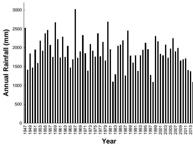
Figure 7. Top left : total annual rainfall data for Penrhyn in the northern Cook Islands from 1951 – 2011. Top right : Kruskal-Wallis analysis of Penrhyn’s monthly rainfall data for the two periods, with p < 0.05 indicating significant difference. Bottom left : total annual rainfall data for Rarotonga in the southern Cook Islands from 1947 – 2013. Bottom right : Kruskal-Wallis analysis of Rarotonga’s monthly rainfall data for the two periods, with p > 0.05 indicating no significant difference.
