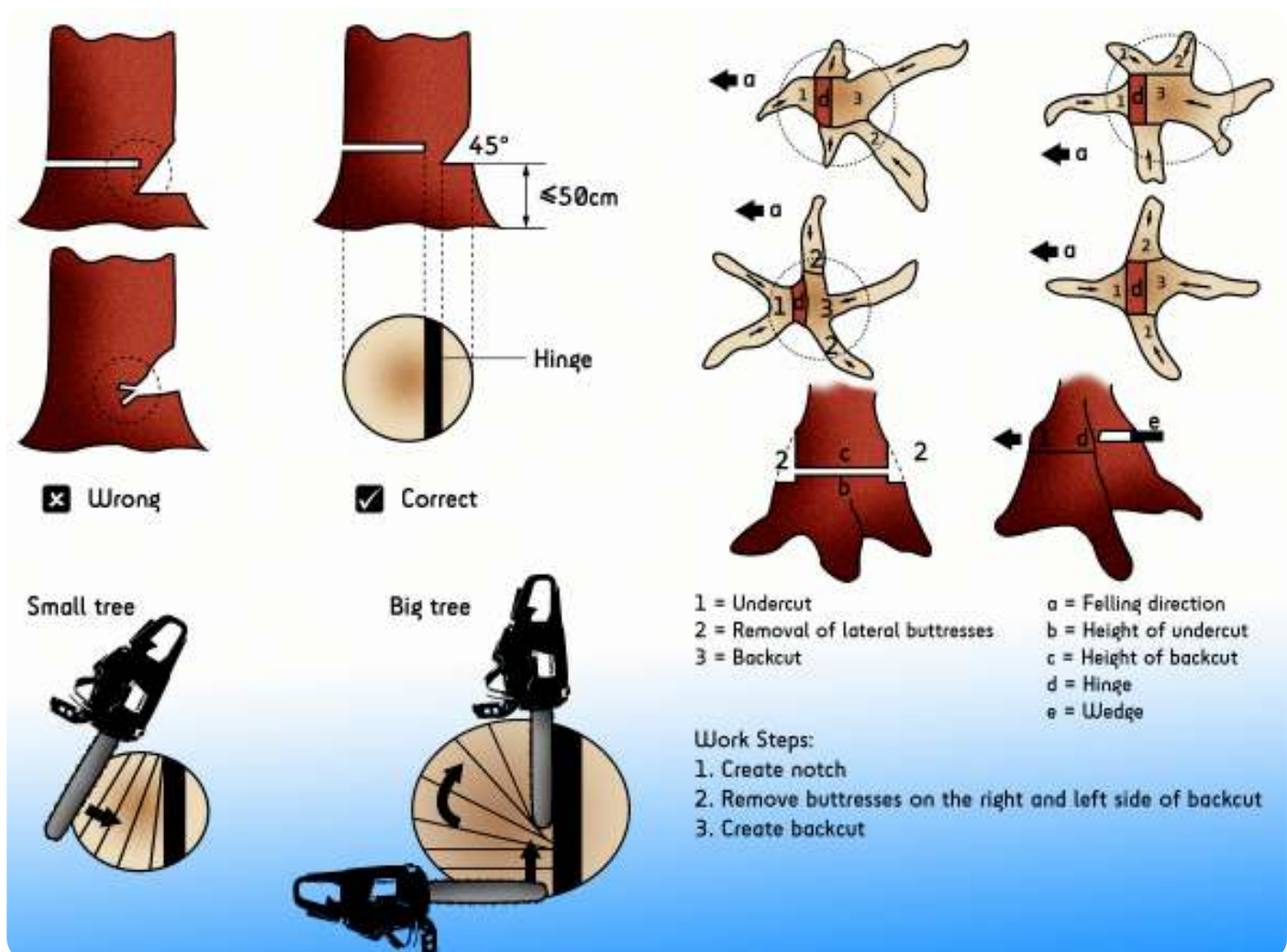
Figure 11.2: Directional felling techniques
