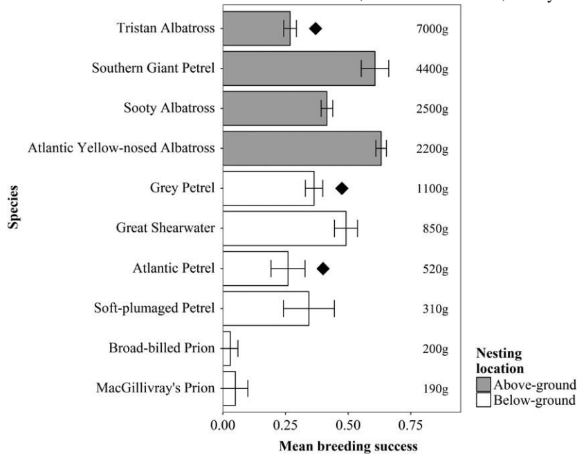
Figure 1.in order of adult body mass (given, right).Mean breeding success ( se) of above-ground and below-ground breeding seabirds on Gough Island. Species are listed ♦ Winter-breeding species (all others breed in the summer).
