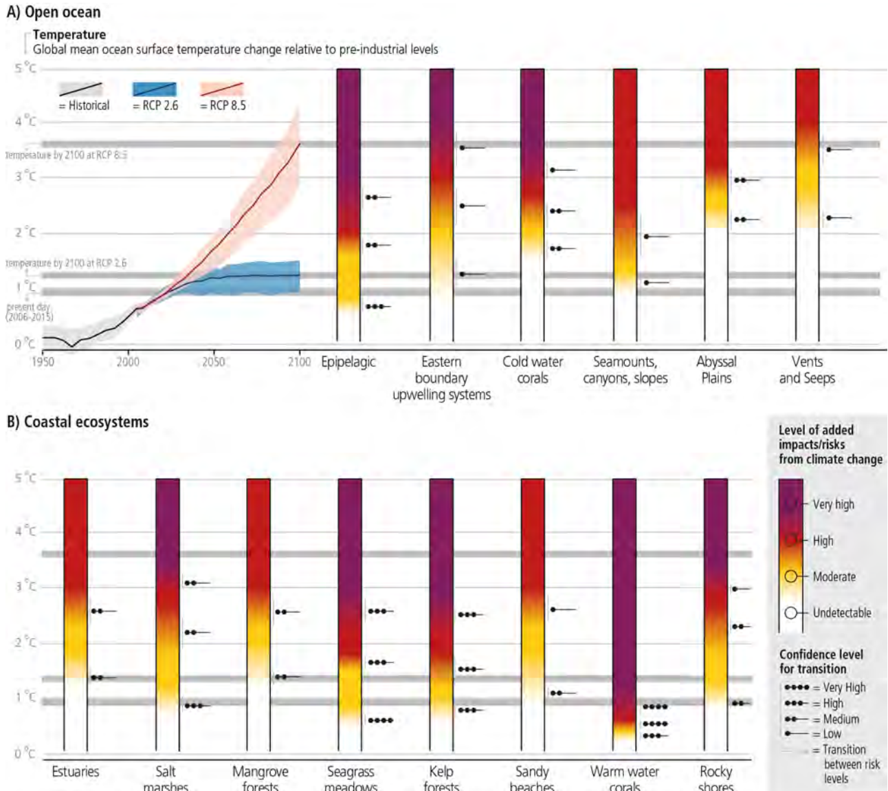
8 9 Figure 5.16: Risk scenarios for open ocean (upper panel) and coastal (lower panel) ecosystems based on observed and 10 projected climate impacts. ‘Present day’ corresponds to the 2000s, whereas the different greenhouse emissions 11 scenarios: RCP2.6 and RCP8.5 correspond to year 2100. Multiple climatic hazards are considered, including ocean 12 warming, deoxygenation, acidification, changes in nutrient, particulate organic carbon flux and sea level rise (see 13 sections 5.2 and 5.3). The projected changes in sea surface temperature (SST) from an ensemble of general circulation 14 models (left panels) indicates the level of ocean changes under RCP2.6 and RCP8.5 (see Cross Chapter Box 1 Table 15 CB1 for the projected global average changes in average air temperature, SST and other selected ocean variables). 16 Global average impacts/risks are represented. Regional variations of risks/impacts are described in Section 5.2.5, 5.3.7 17 and the Supplementary Material (SM5.2 and SM5.5). Impact/risk levels do not consider human risk reduction strategies 18 such as societal adaptation, or future changes in non-climatic hazards. The grey vertical bars indicate the transition 19 between the levels of risks, with their confidence level based on expert judgment. Note: The figure depicts climate 20 change impacts and risks on warm water corals taken from SR1.5, based on global models. Observed impacts on coral 21 reefs ecosystems outlined in Section 5.3.4 and Box 5.5 reveal a more complex situation that may result in regional 22 differences in confidence levels. 23 24
