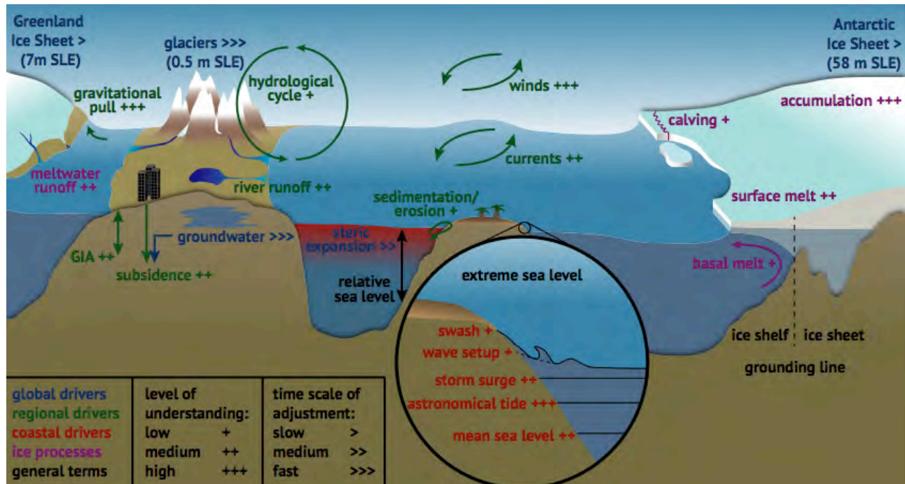
Figure 4.4: A schematic illustration of the climate and non-climate driven processes that can influence global, regional (green colours), relative and extreme sea level events (red colors) along coasts. Major ice processes are shown in purple and general terms in black. SLE stands for Sea Level Equivalent and reflects the increase in GMSL if the mentioned ice mass is melted completely and added to the ocean.
