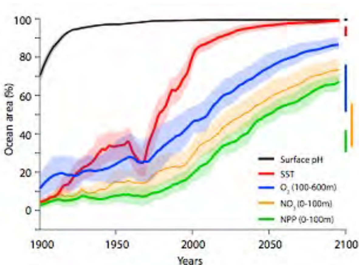
Box 5.1, Figure 1: Time of emergence of key ocean condition variables: sea surface temperature (SST), surface pH, 100-600m oxygen (O 2 ), 0-100m nitrate (NO 3 ), and 0-100m integrated net primary production (NPP). The year of emergence represents the year when the mean change relative to the reference period of 1986-2005 is above the standard deviation of each variable over the historical period (Frölicher et al., 2016) and is expressed here in terms of the rate at which different climate signals emerge as a proportion of total ocean area for the RCP8.5 scenario. The final area (and standard deviation) by 2100 under the RCP2.6 scenario is indicated by vertical lines at 2100.
