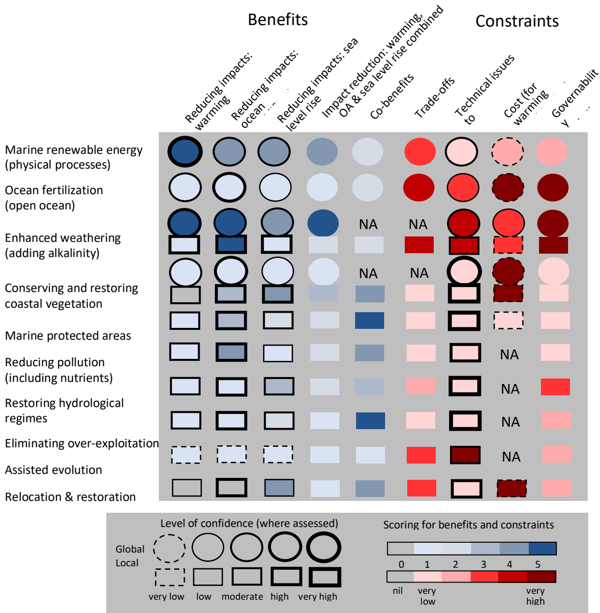
Figure 5.23: Summary of potential benefits and constraints of ocean-based risk-reduction options using natural processes, from literature-based expert assessments by Gattuso et al. (2018). Mitigation effectiveness was quantified relative to RCP 8.5, assuming maximum theoretical implementation, with reduction of climate-related drivers considered at either global or local (< 100 km 2 ) scale, shown as circles or rectangles respectively. Impact reduction, co-benefits and trade-offs are in the context of eight sensitive marine ecosystems and ecosystem services. ‘Technical issues to overcome’ is based on scores for technological readiness, lead time for full implementation and duration of effects. Cost is based on USD per tonne of CO 2 either not released or removed from the atmosphere (for global measures) or per hectare of coastal area with action implemented (for local measures). ‘Governance challenges’ shows the potential difficulty of implementation by the international community. NA, not assessed. Additional information on scoring methods is given in Supplementary Material SM5.4, Tables SM5.9a and SM5.9b.
