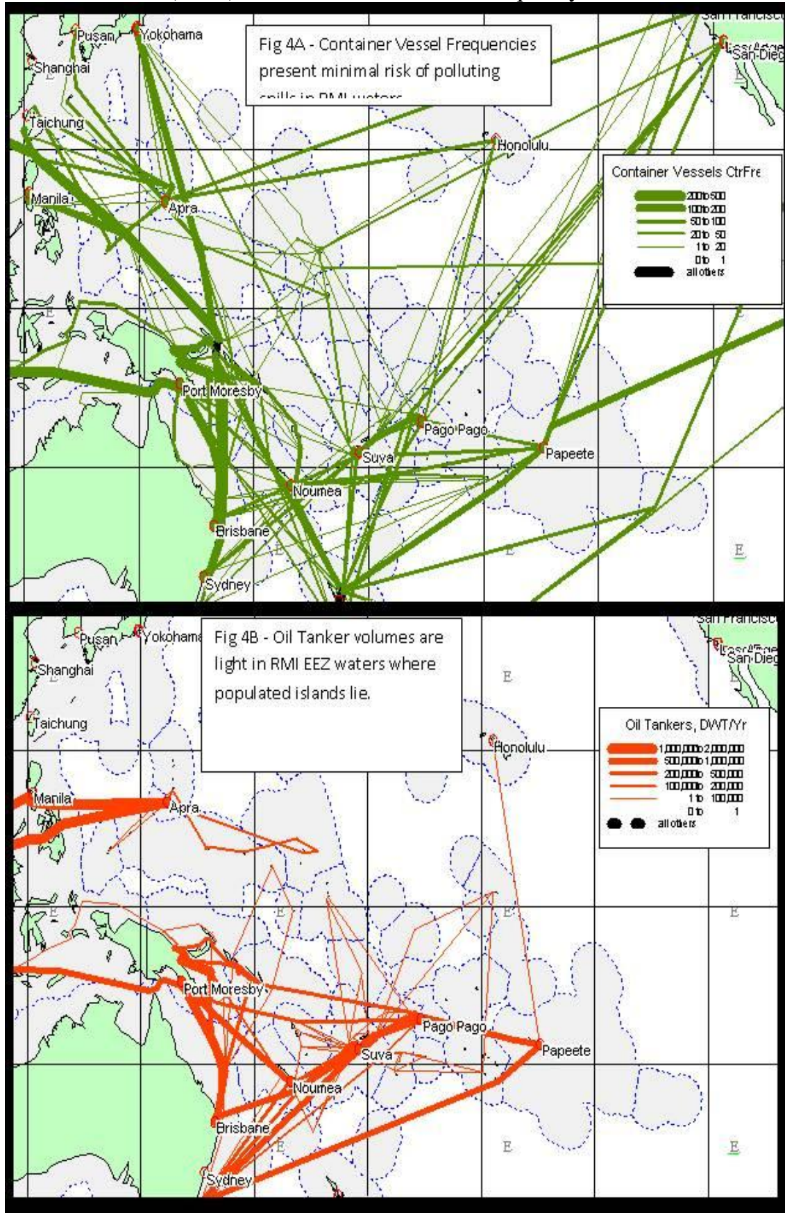
FIGURE FOUR (A&B) Oil Tanker & Container Frequency Charts
