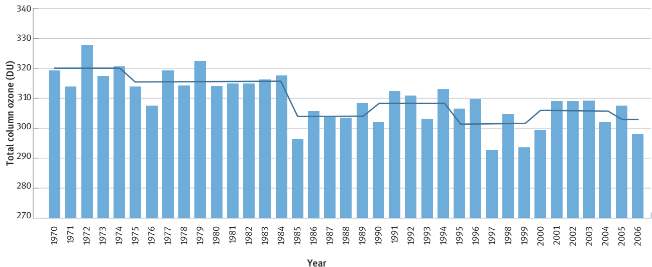
+ FIGURE 3.3: AVERAGE YEARLY OZONE LEVELS OVER NEW ZEALAND, 1970–2006
