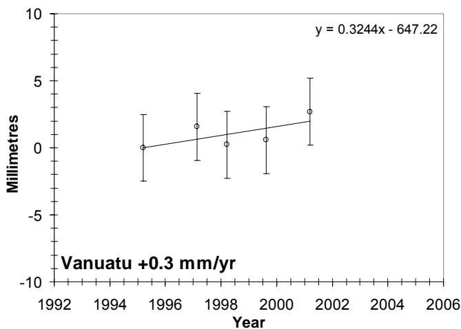
Figure 28. Movement of the SEAFRAME Sensor relative to the Tide Gauge Bench Mark
