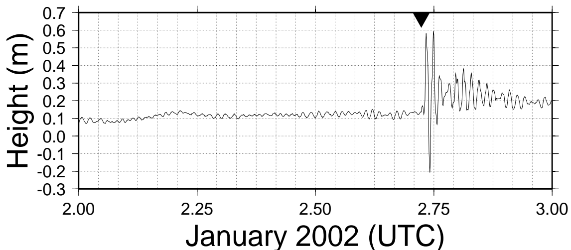
Figure 17. Port Vila sea level response to Jan 2002 Vanuatu Earthquake
