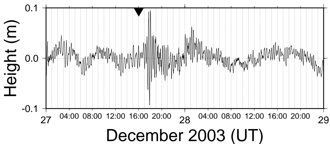
Figure 18. Port Vila sea level response to Dec 2003 Vanuatu Earthquake
