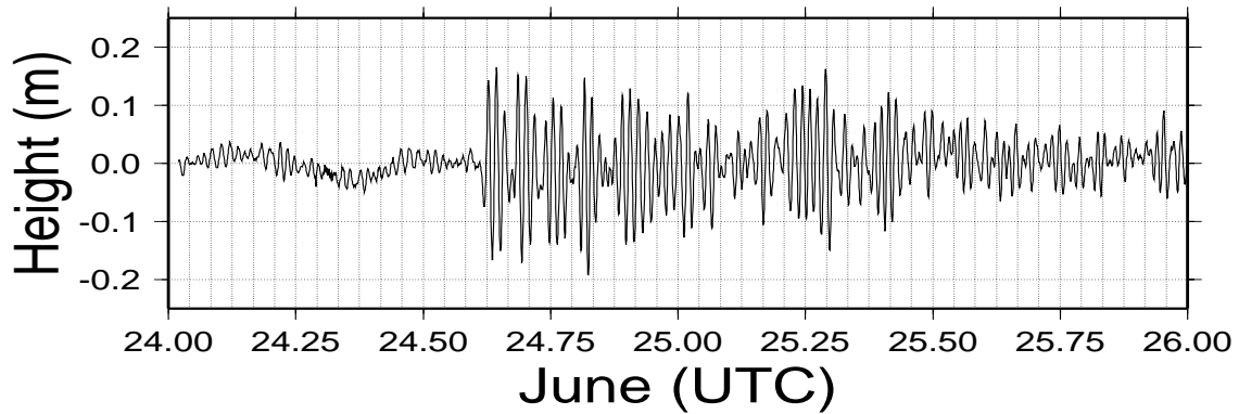
Figure 14. The non-tidal sea level record (m) at Vanuatu following a tsunamigenic earthquake off Peru at 20:33 UTC on 23 June 2001.
