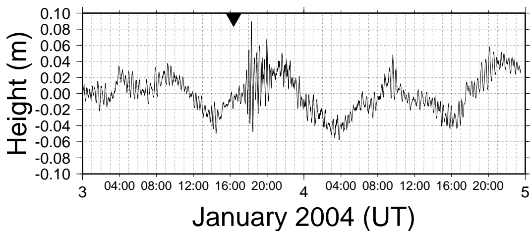
Figure 19. Port Vila sea level response to Jan 2004 Vanuatu Earthquake
