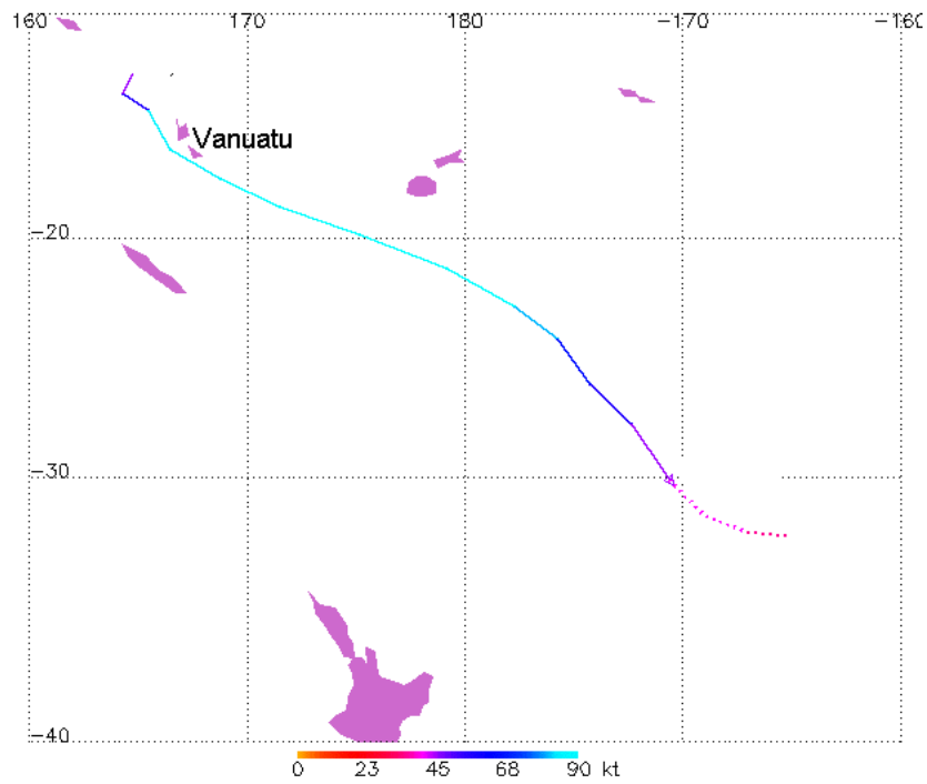
Figure 10. Track of Tropical Cyclone Paula, February/March 2001
