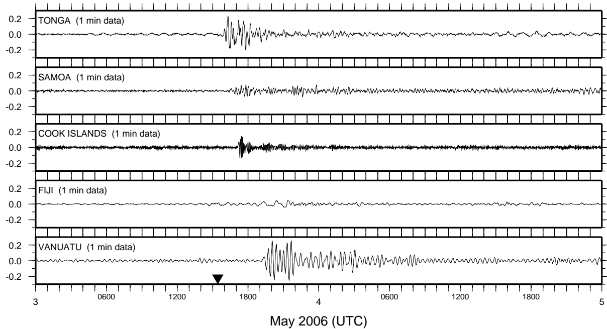
Figure 20. The non-tidal sea level record (m) at SEAFRAME stations following a tsunamigenic earthquake near Tonga at 15:27 UTC on 3 May 2006.
