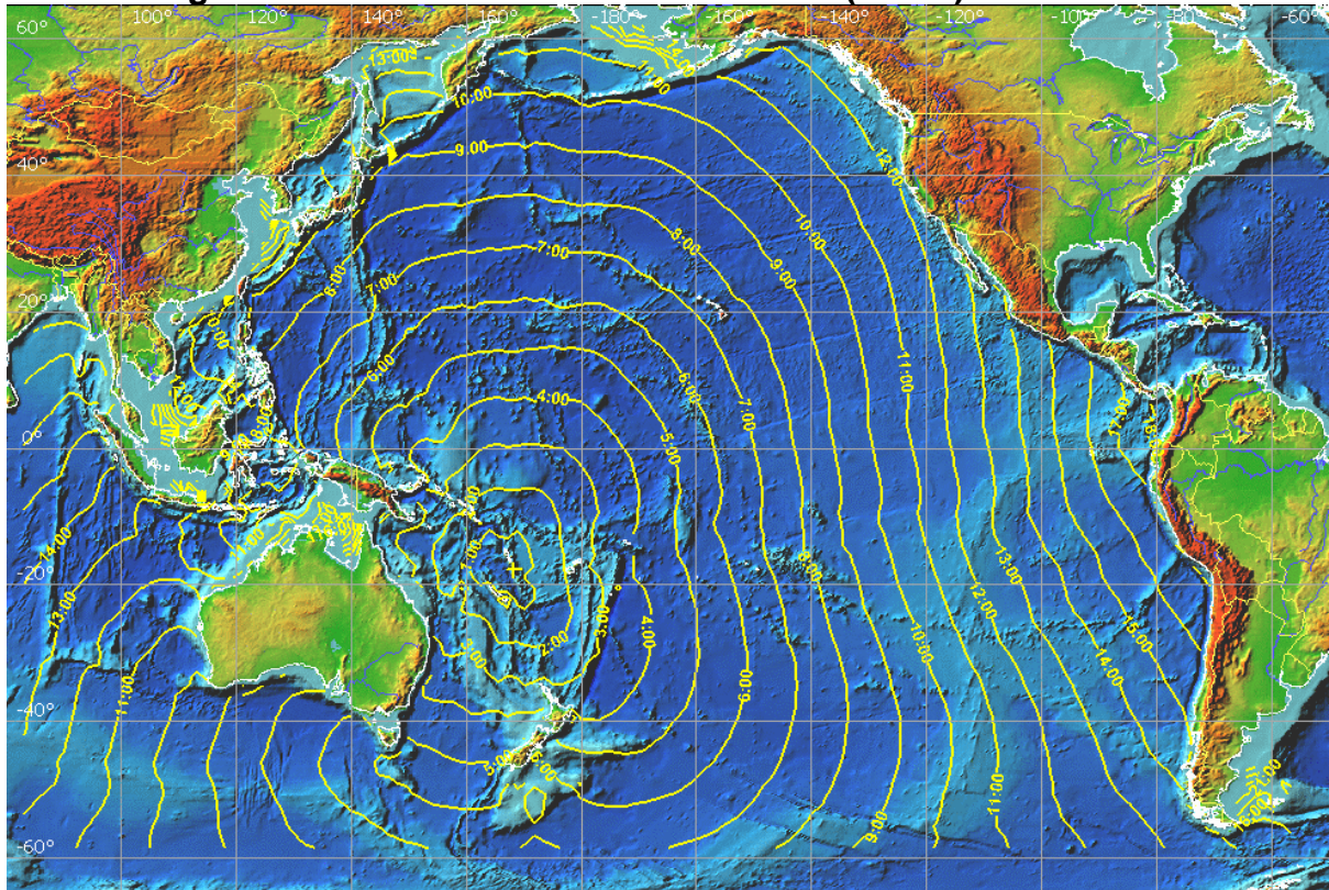
Figure 13. Inverse Tsunami Travel Times (hours) for Vanuatu.
