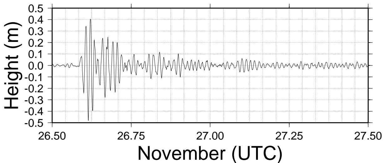
Figure 16. Port Vila sea level response to Nov 1999 Vanuatu Earthquake
