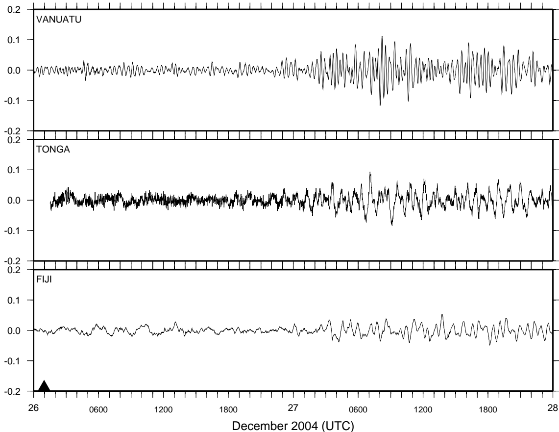
Figure 15. Non-tidal Sea Level Signal (m) following the 26 December 2004 Indian Ocean Earthquake.
