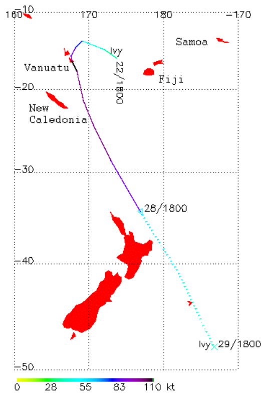
Figure 11. Track of Tropical Cyclone Ivy, February 2004
