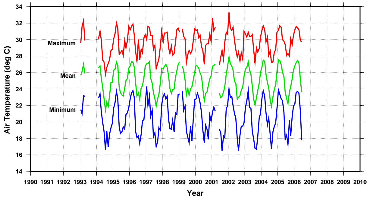
Monthly air temperature at Port Vila SEAFRAME gauge
