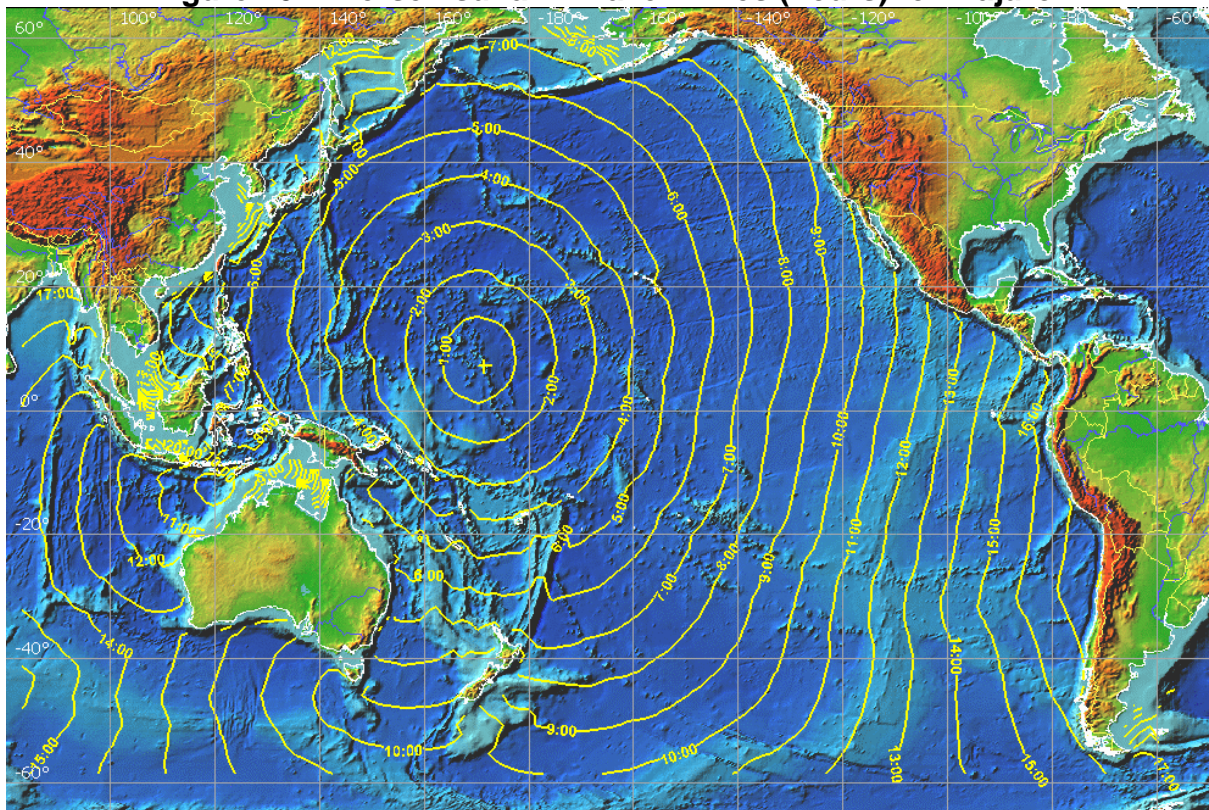
Figure 10. Inverse Tsunami Travel Times (hours) for Majuro.
