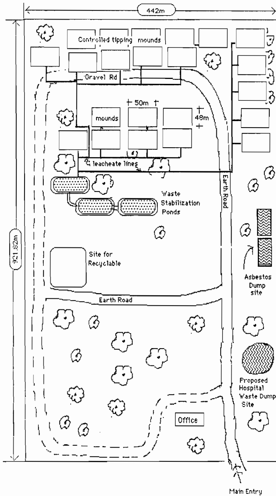
Fig. 4: Proposed layout of Tafaiyata dump site.
