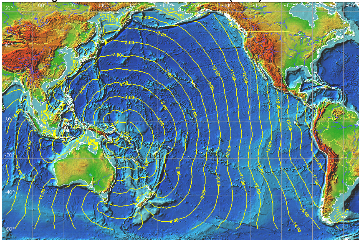
Figure 10. Inverse Tsunami Travel Times (hours) for Honiara.
