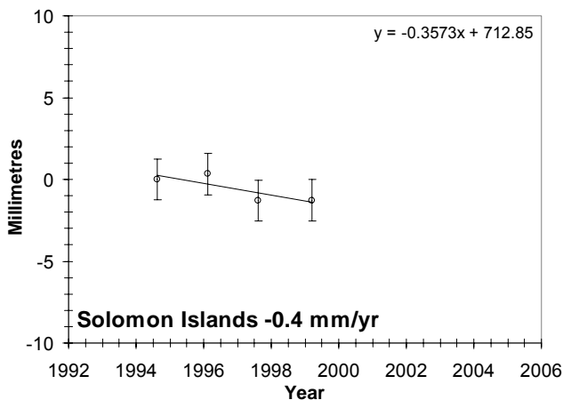
Figure 18. Movement of the SEAFRAME Sensor relative to the Tide Gauge Bench Mark.
