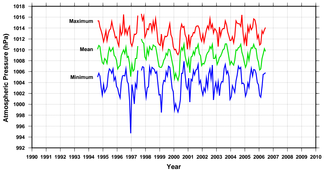
Monthly atmospheric pressure at Honiara SEAFRAME gauge
