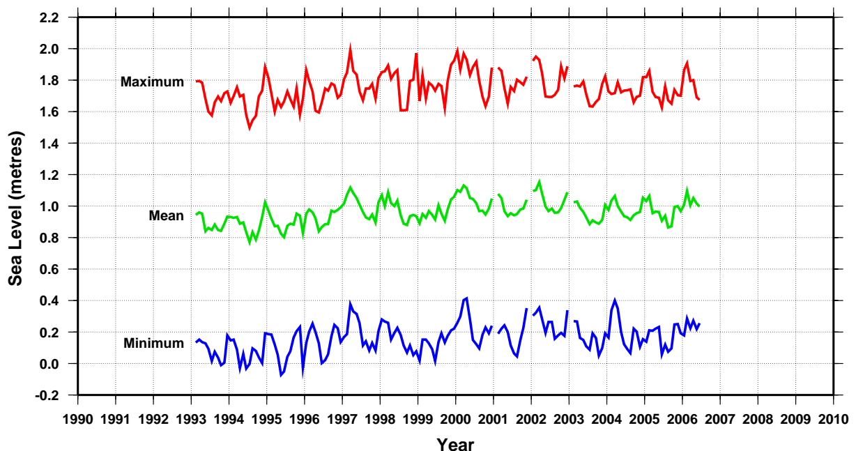
Monthly sea level at Nuku'alofa SEAFRAME gauge
