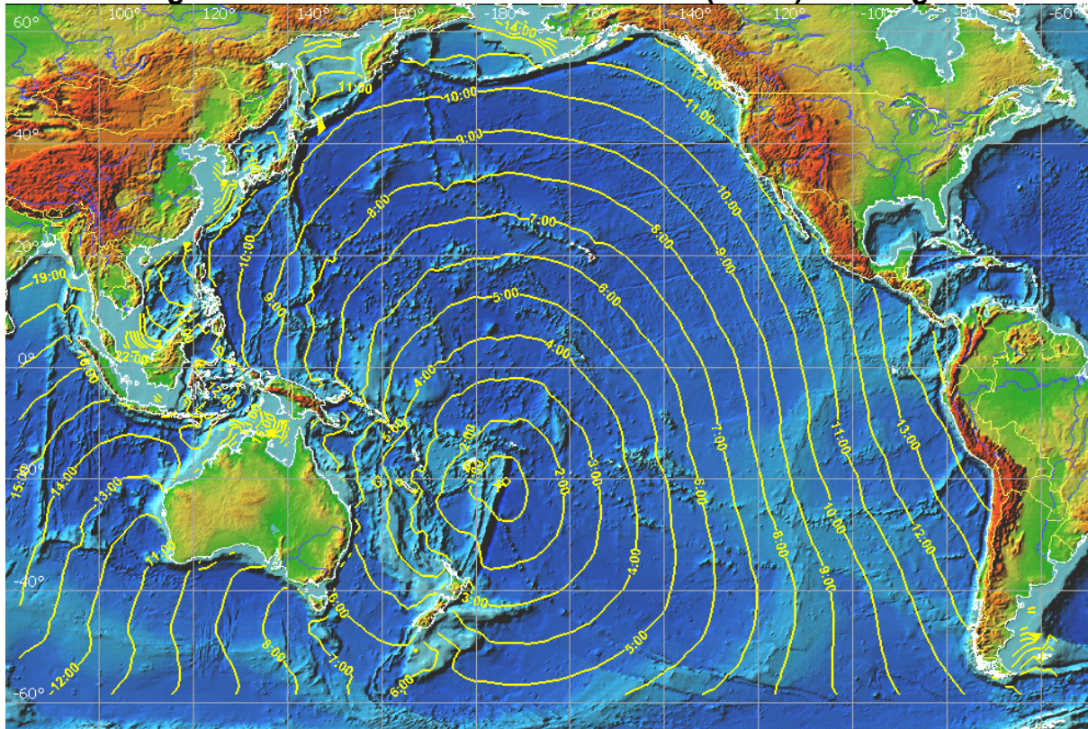
Figure 12. Inverse Tsunami Travel Times (hours) for Tonga.
