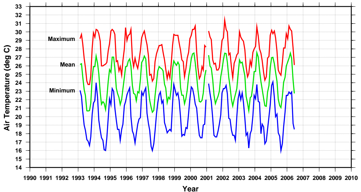
Monthly air temperature at Nuku'alofa SEAFRAME gauge
