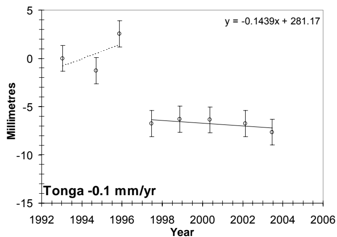
Figure 23. Movement of the SEAFRAME Sensor relative to the Tide Gauge Bench Mark.
