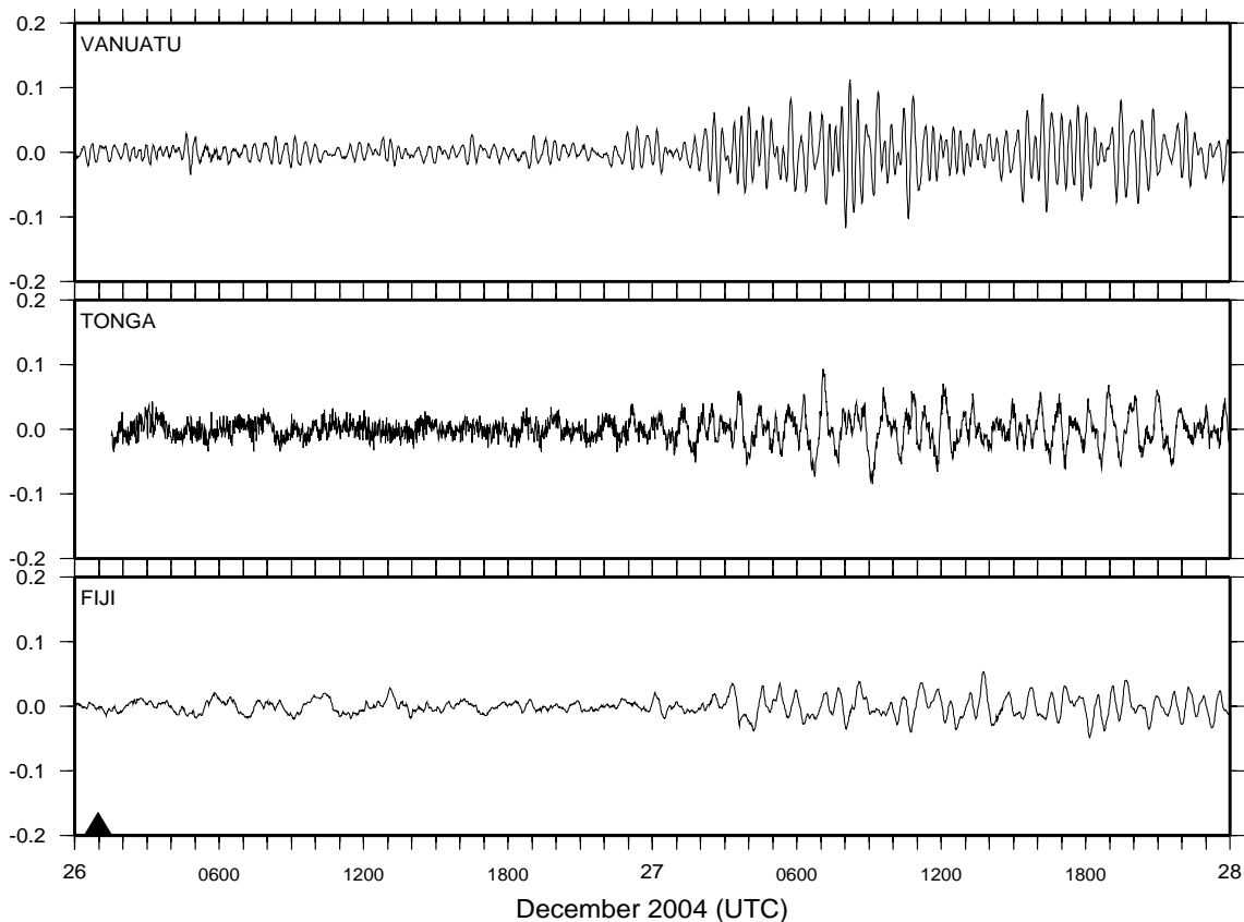
Figure 14. Non-tidal Sea Level Signal (m) following the 26 December 2004 Indian Ocean Earthquake.
