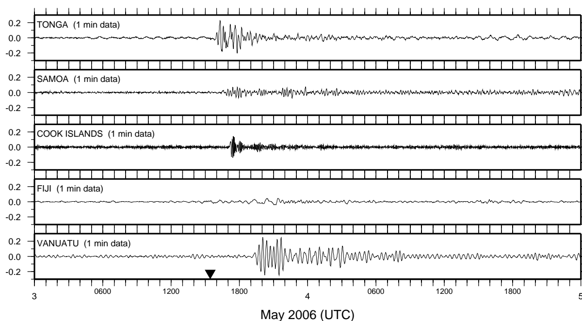
Figure 15. The non-tidal sea level record (m) at SEAFRAME stations following a tsunamigenic earthquake near Tonga at 15:27 UTC on 3 May 2006.
