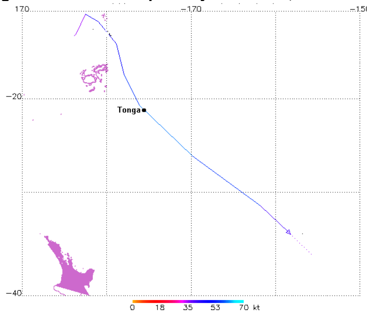
Figure 9. Track of Tropical Cyclone Hina, March 1997
