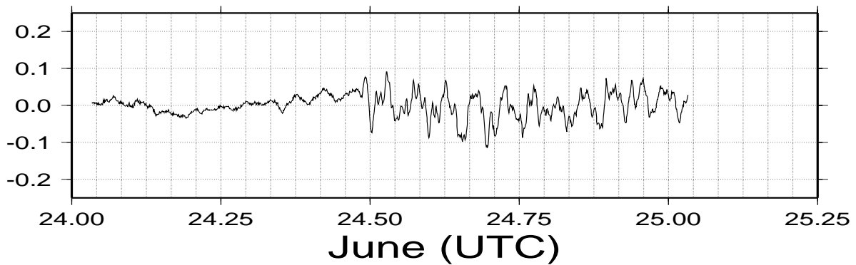
Figure 13. The non-tidal sea level record (m) at Tonga in June 2001 following a tsunamigenic earthquake off Peru.
