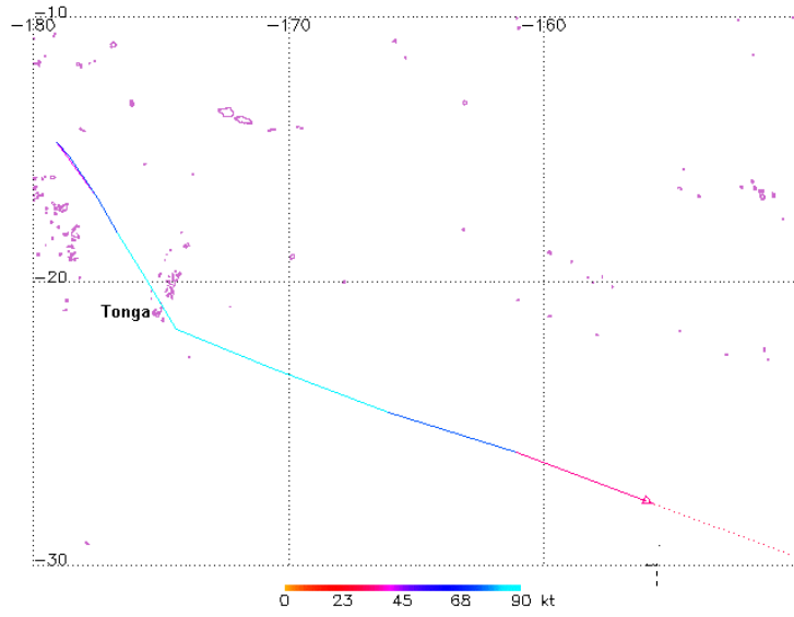
Figure 10. Track of Tropical Cyclone Cora, December 1998
