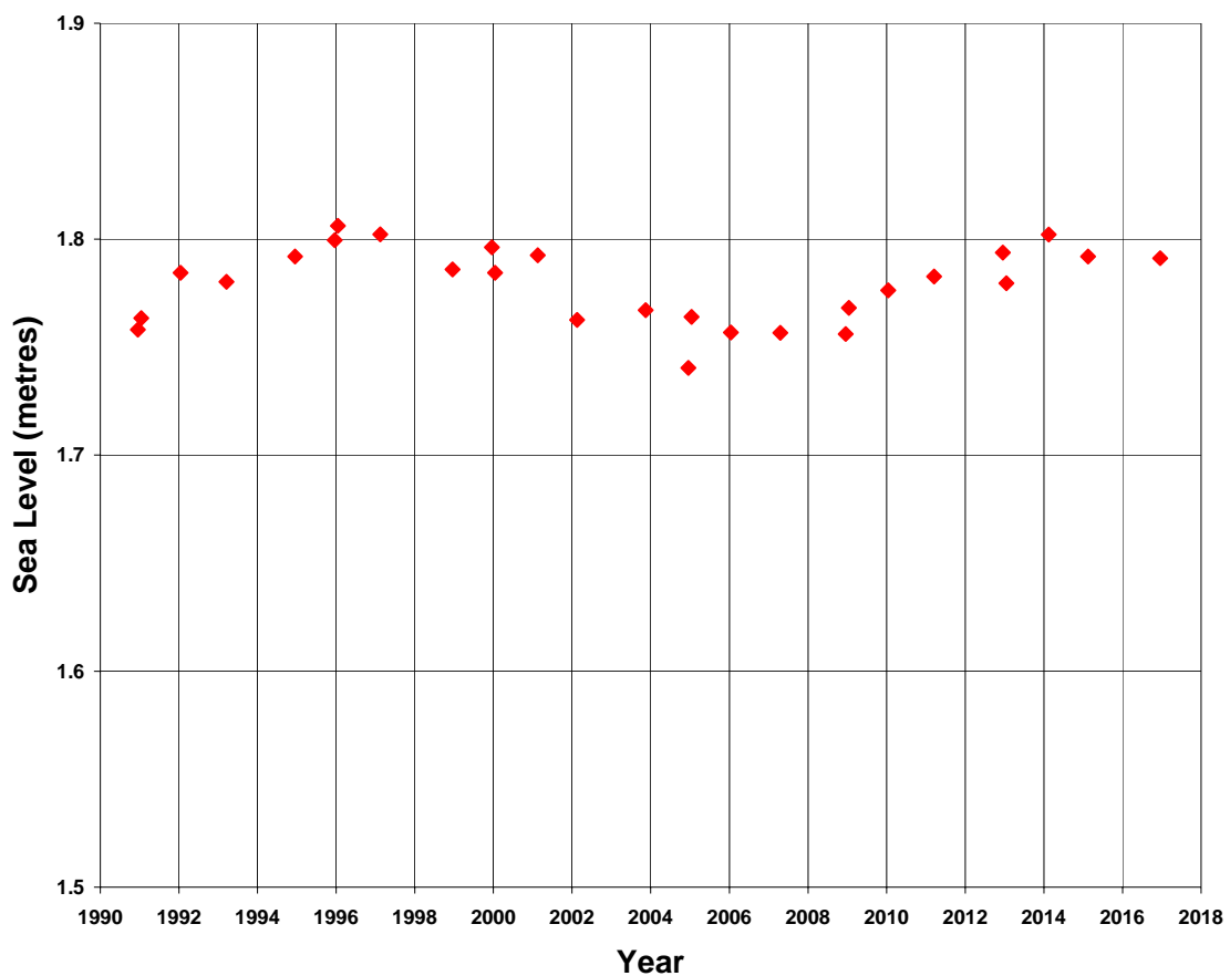
Predicted highest tide each year for Nuku' Alofa
