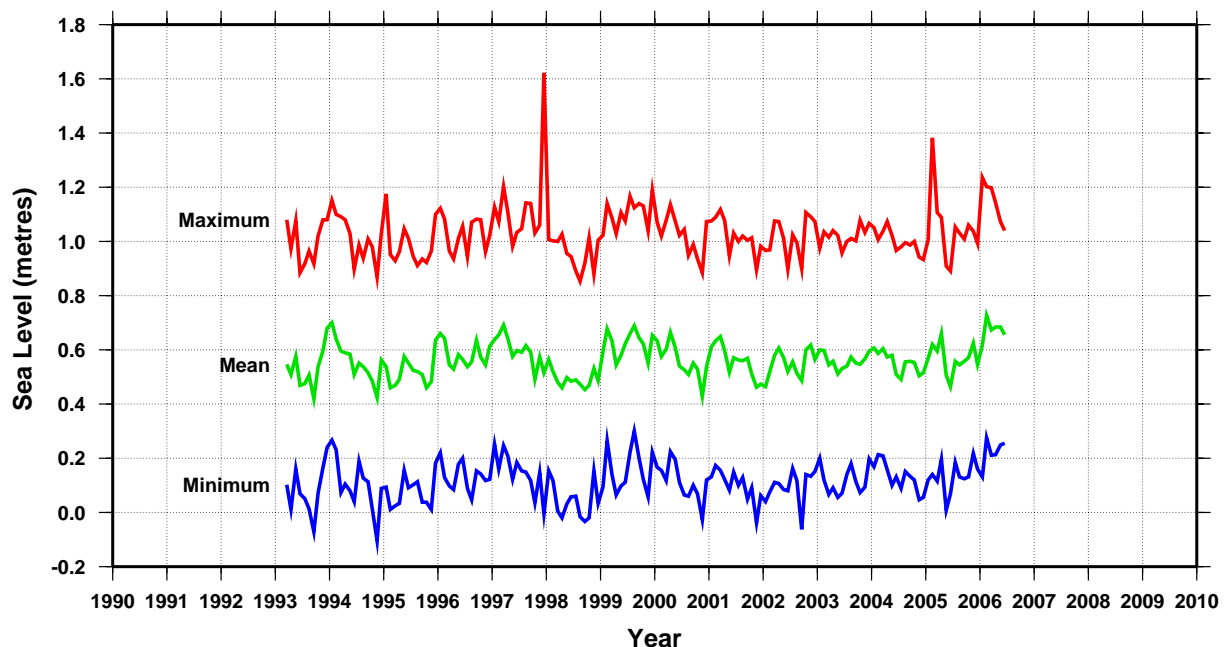
Monthly sea level at Avatiu SEAFRAME gauge
