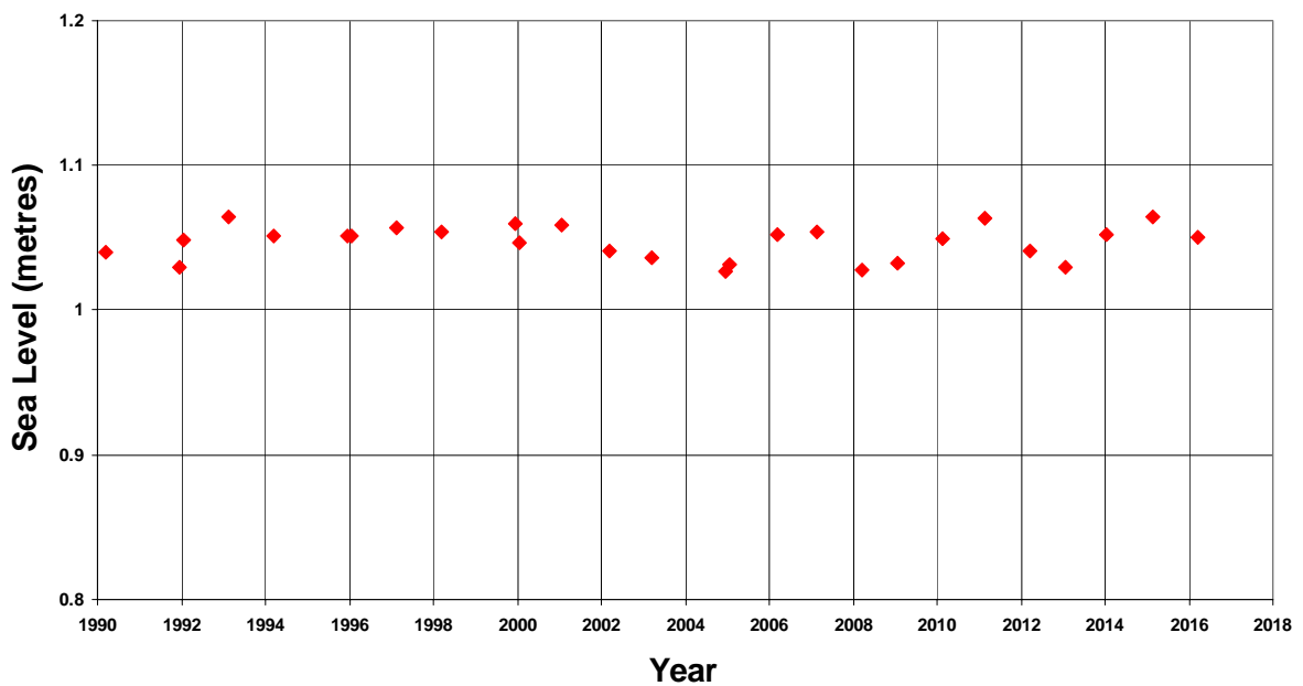
Figure 17 Predicted highest tide each year for Avatiu
