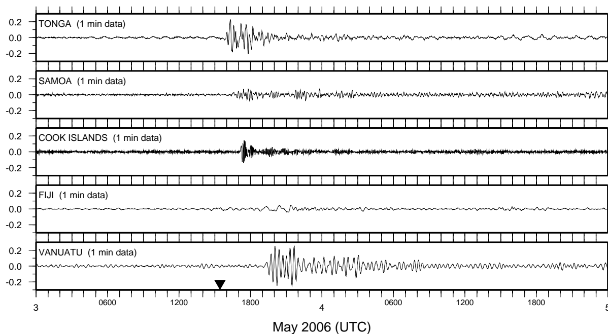
Figure 12. The non-tidal sea level record (m) at SEAFRAME stations following a tsunamigenic earthquake near Tonga at 15:27 UTC on 3 May 2006.
