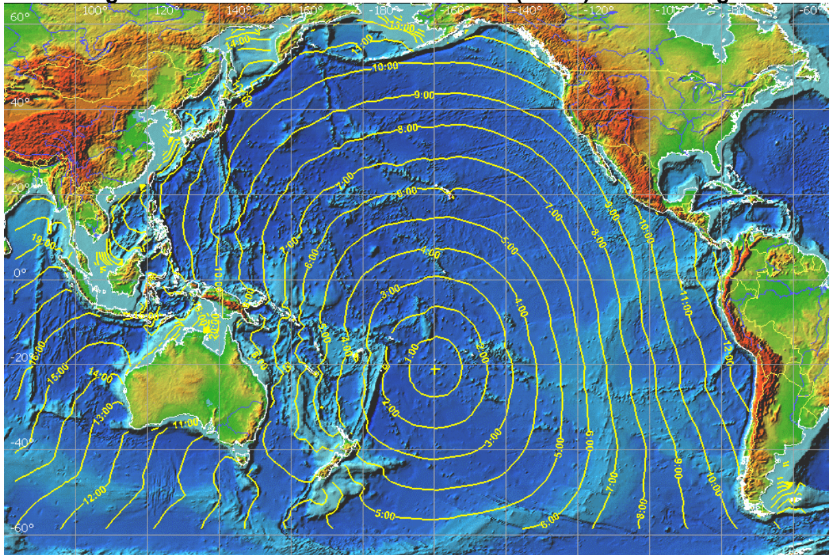
Figure 10. Inverse Tsunami Travel Times (hours) for Rarotonga.
