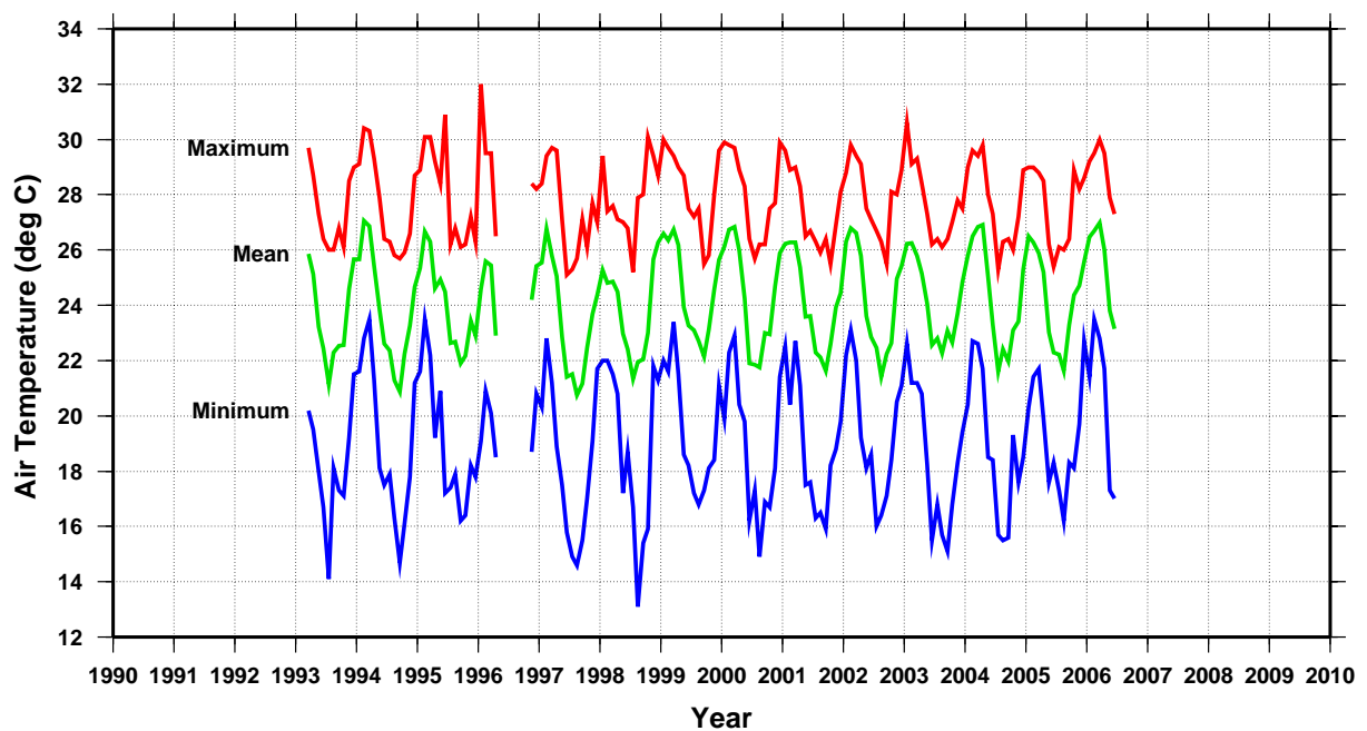
Monthly air temperature at Avatiu SEAFRAME gauge
