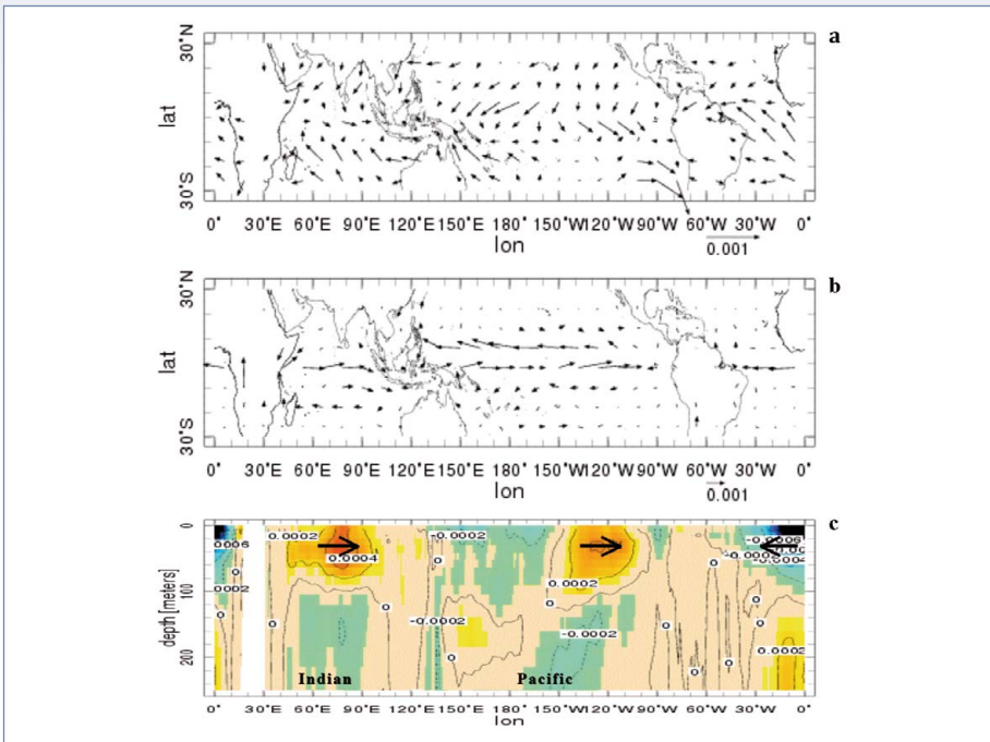
Figure 6. (a) Trends in wind stress in 1958–2007 ( \text{N}/\text{m}^2/\text{yr} ), related to the square of wind speed (from the European Centre for Medium-Range Weather Forecasts). Trends in currents in 1958–2007 ( \text{m}/\text{s}/\text{yr} ): (b) 1–200 m depth averaged map; (c) east–west section averaged 30° N–30° S ( http://iridl.ldeo.columbia.edu ).
