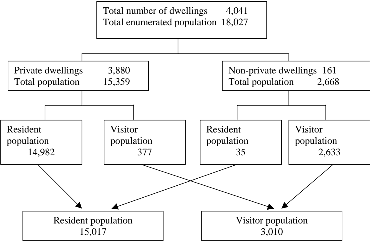
Figure 2: Population composition
