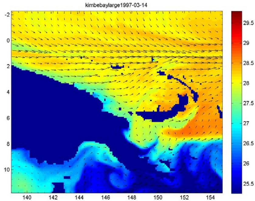
Figure 33. Model 1997-03-14.
