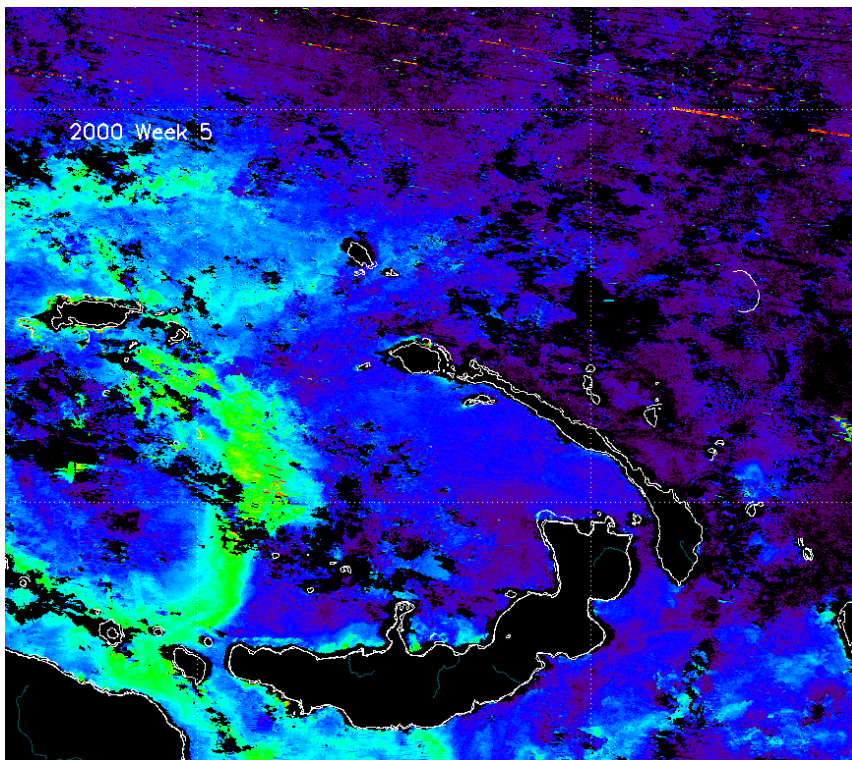
Figure 13. SeaWiFS 2000 Week 5.
