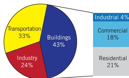
CO 2 Emissions from Fossil Fuel Combustion by End-Use Sector, 2006
