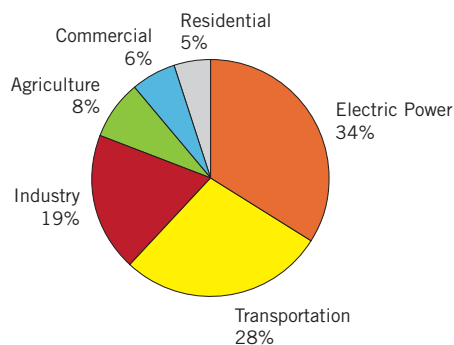
U.S. GHG Emissions by Sector in 2006
