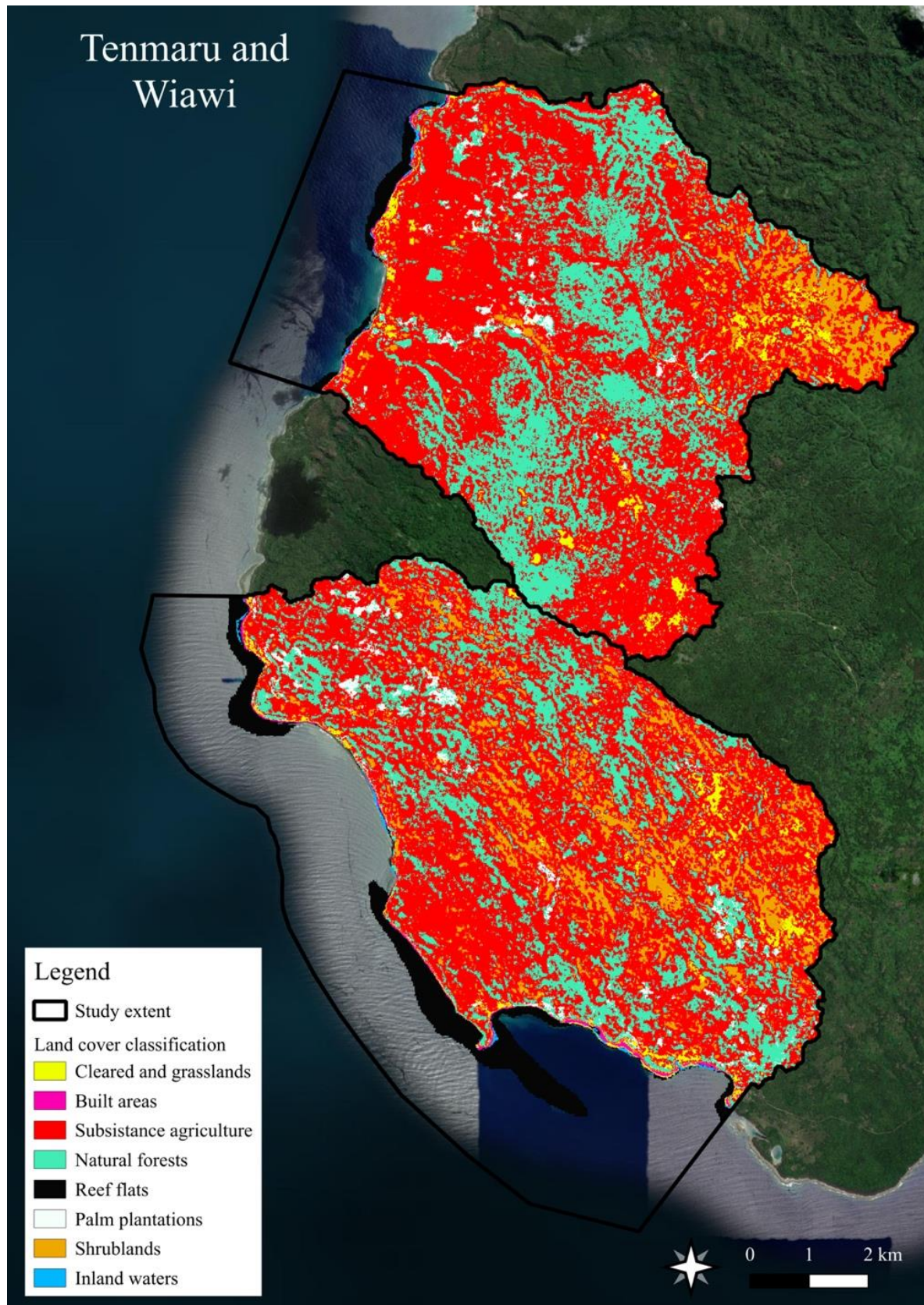
Figure 3: Land cover and ecosystem type for Tenmaru (to the north) (and Wiawi) area of interest.
