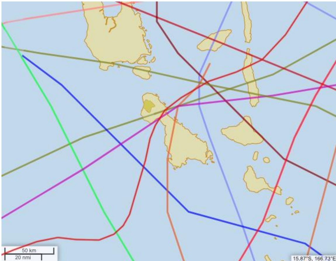
Figure 2: Tropical cyclone activity for Tenmaru (shaded) between 2001-2023).
