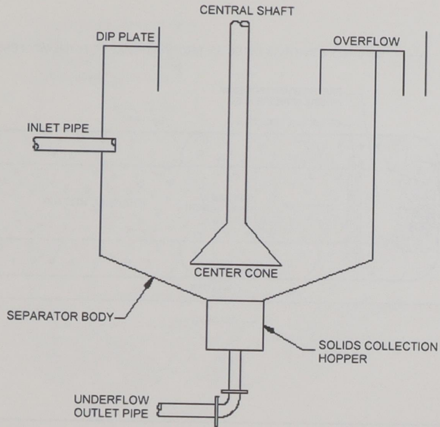
Figure 3.19 Hydrodynamic Device (LA-5)
