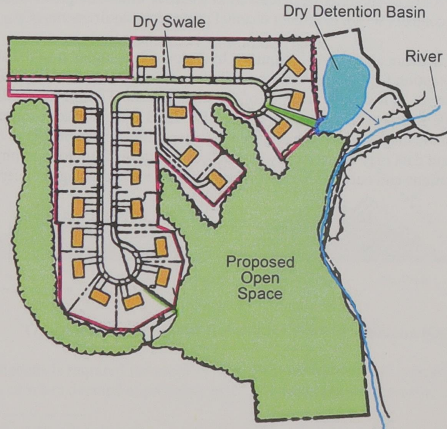
Figure 2.7 Medium Density Residential Site Plan in Melekeok
