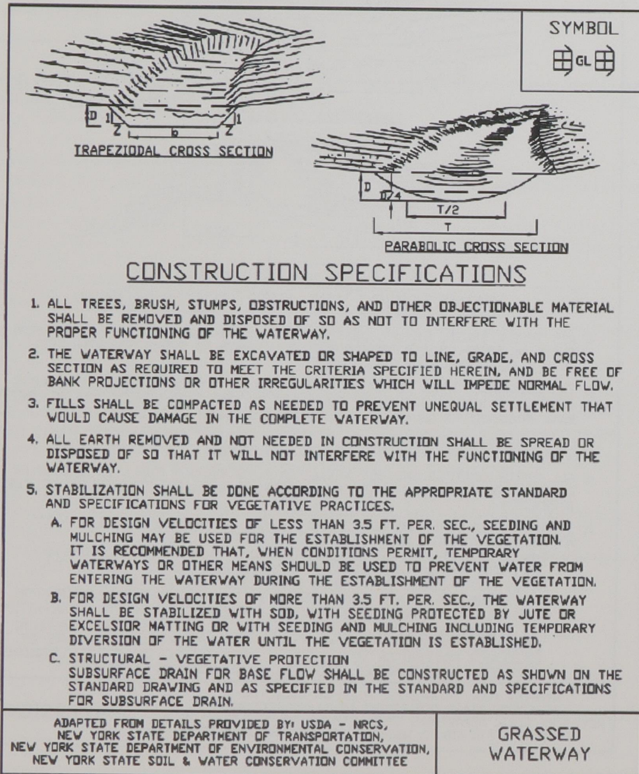
Figure A11.2 Grassed Waterway
