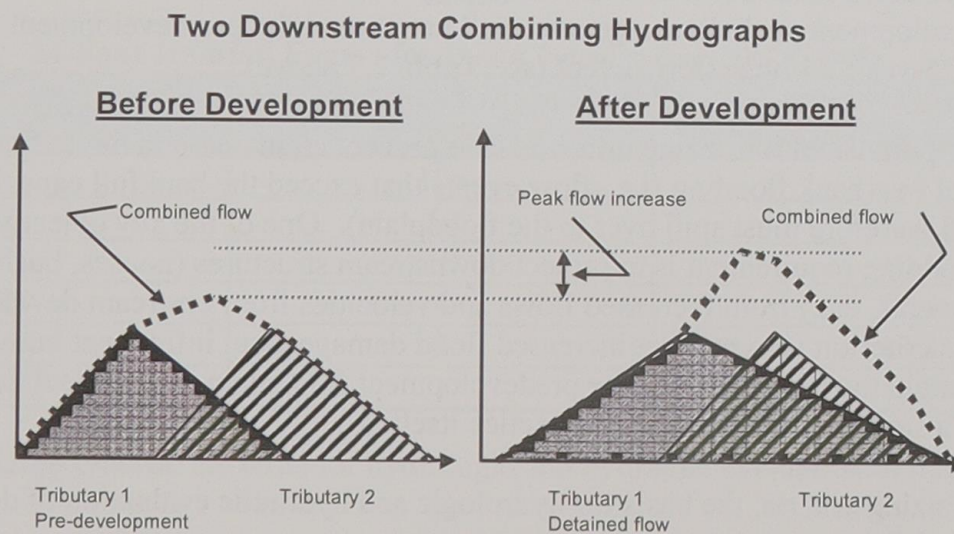
Figure 2.6 Graphical Depictions of Coincident Peak Phenomena (Ogden, 2000)
