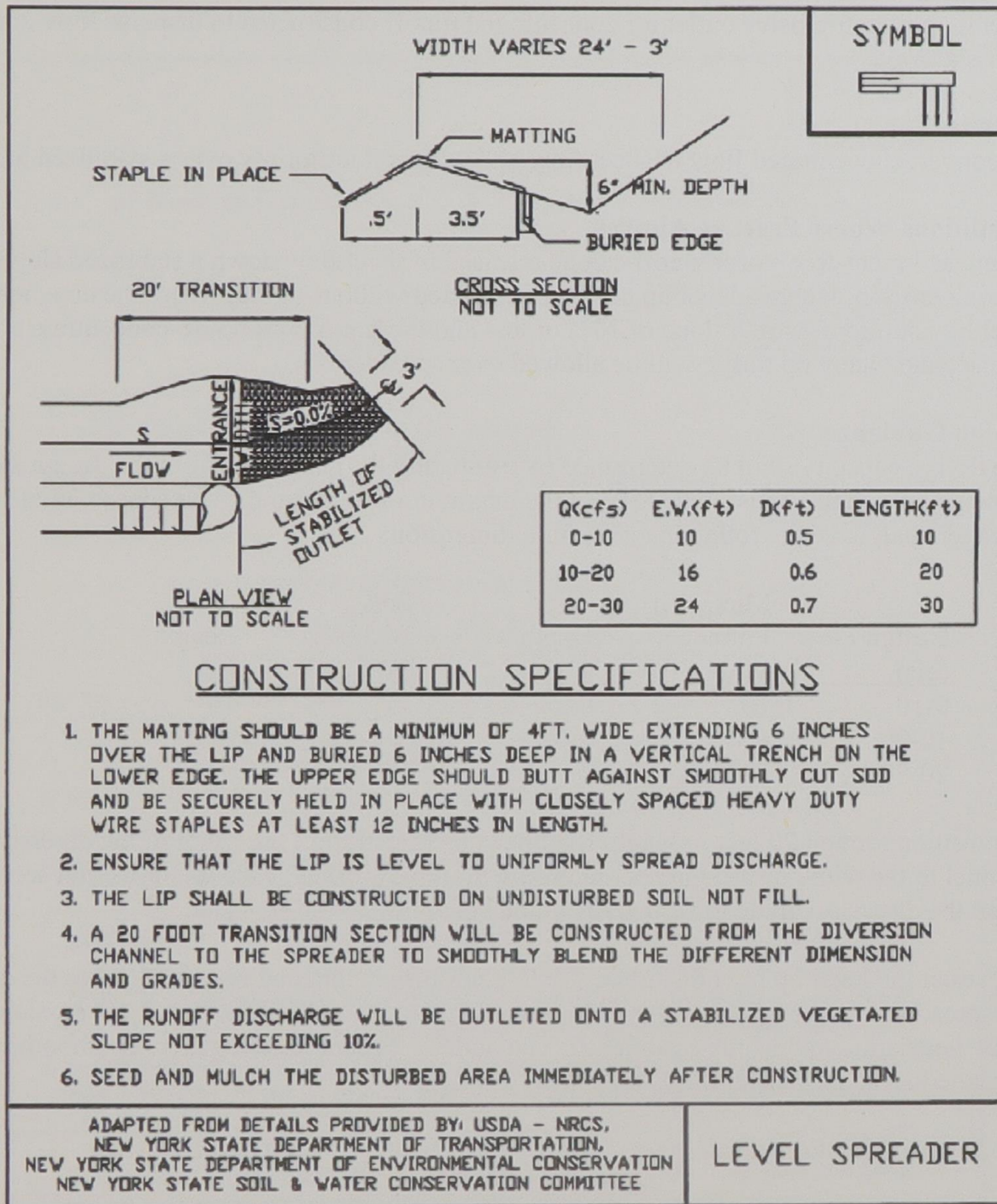
Figure A3.1 Level Spreader
