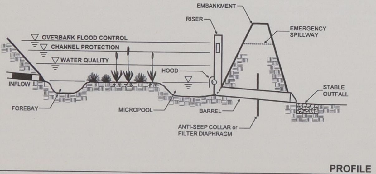
Figure 3.1 Micropool Extended Detention Pond (P-1)
