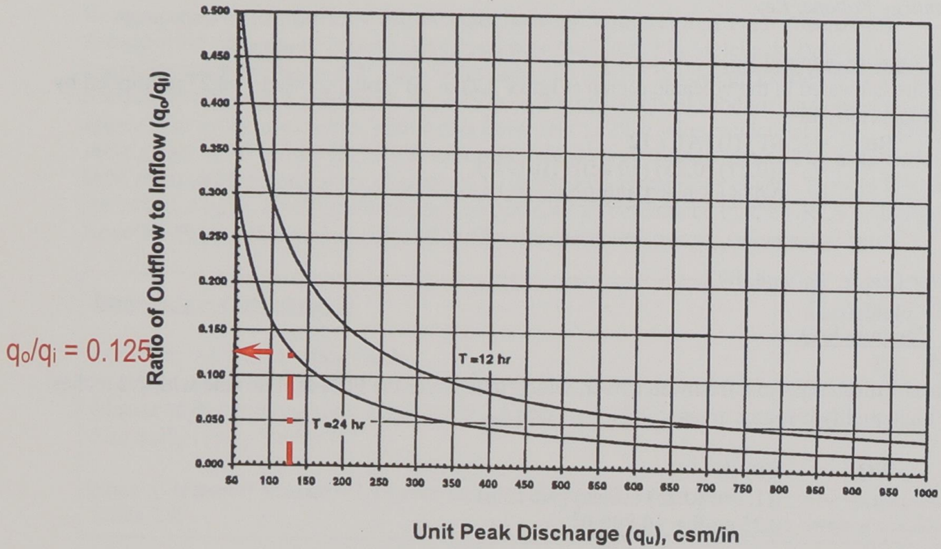
Figure 2.9 Approximate Detention Basin Routing For Rainfall Types I, IA, II, and III. (Source: TR-55, 1986)
