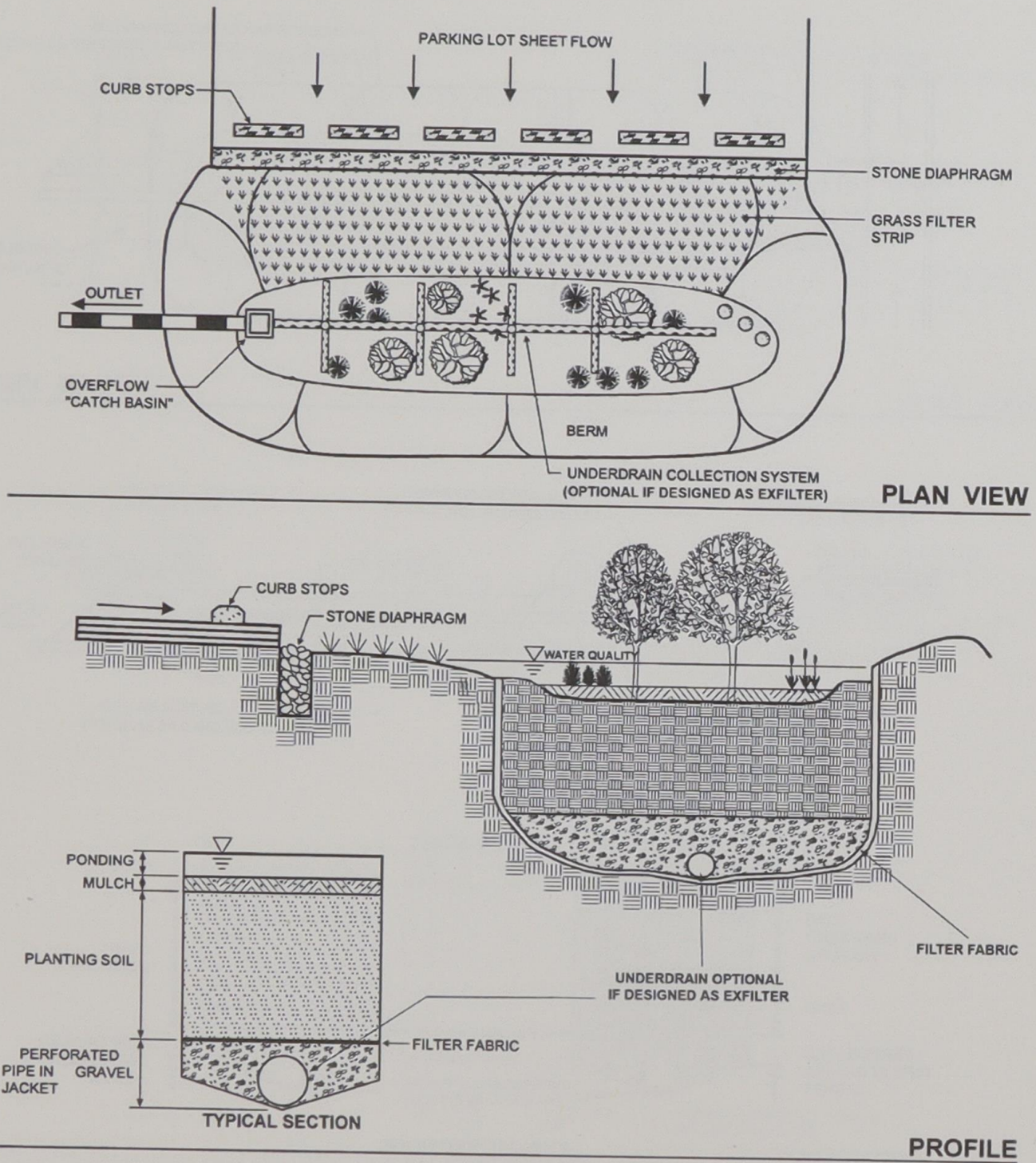
Figure 3.12 Bioretention (F-3)
