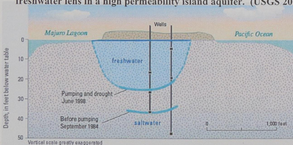
Figure 1.11 Effects of groundwater withdrawal and drought on the potable part of the freshwater lens in a high permeability island aquifer. (USGS 2008, Gordon Tribble)
