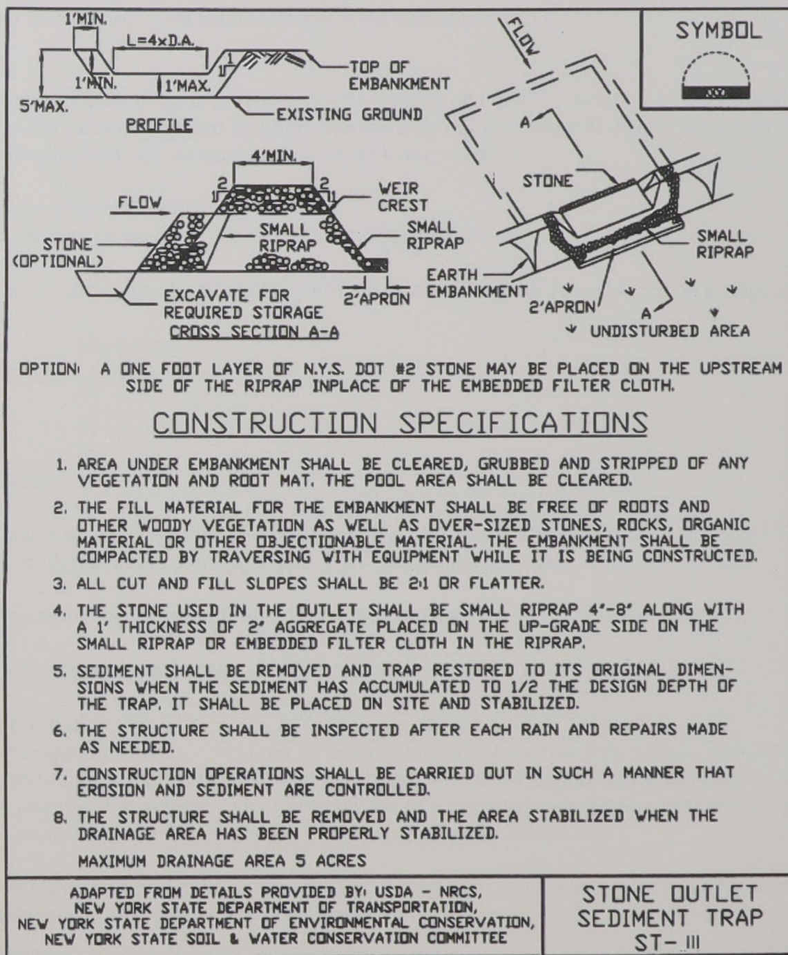
Figure A6.4 Stone Outlet Sediment Trap
