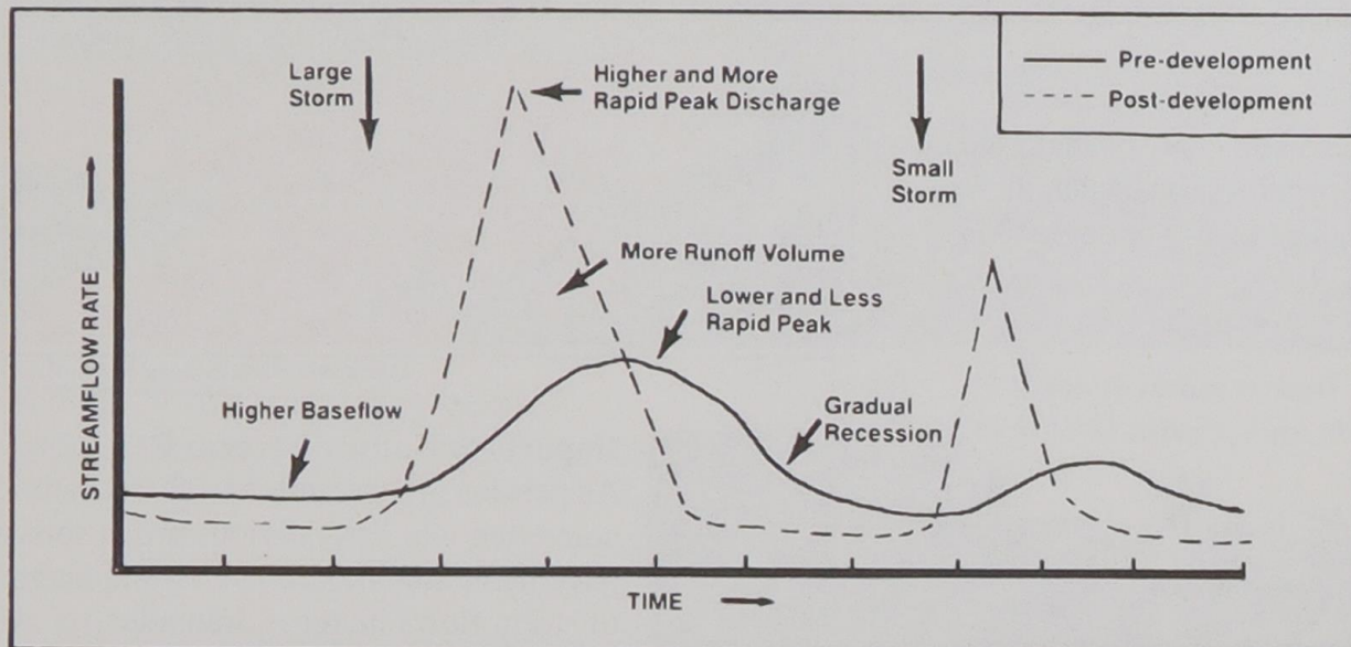
Figure 1.7 Hydrographs Before and After Development
