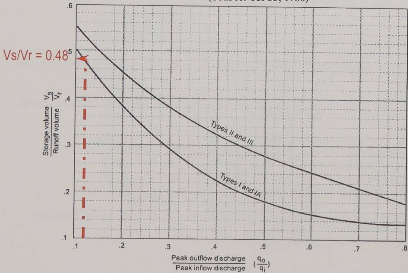
Figure 2.9 Approximate Detention Basin Routing For Rainfall Types I, IA, II, and III. (Source: TR-55, 1986)
