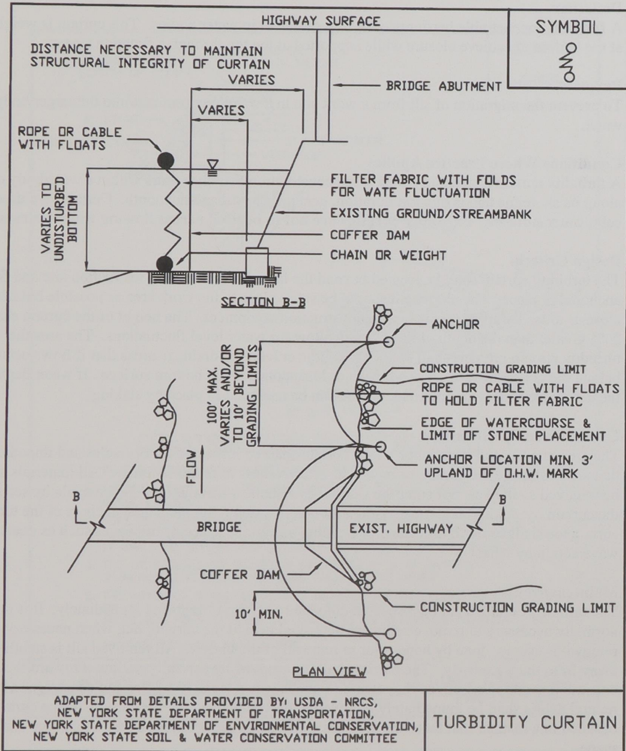
Figure A10.1 Turbidity Curtain
