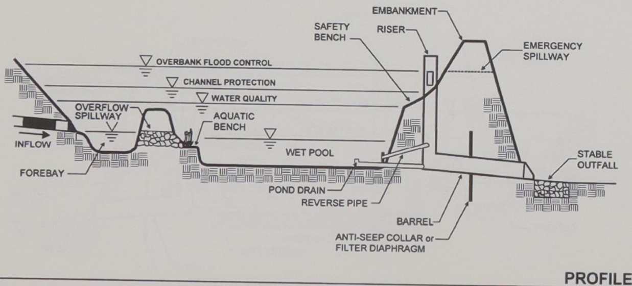
Figure 3.3 Wet Extended Detention Pond (P-3)
