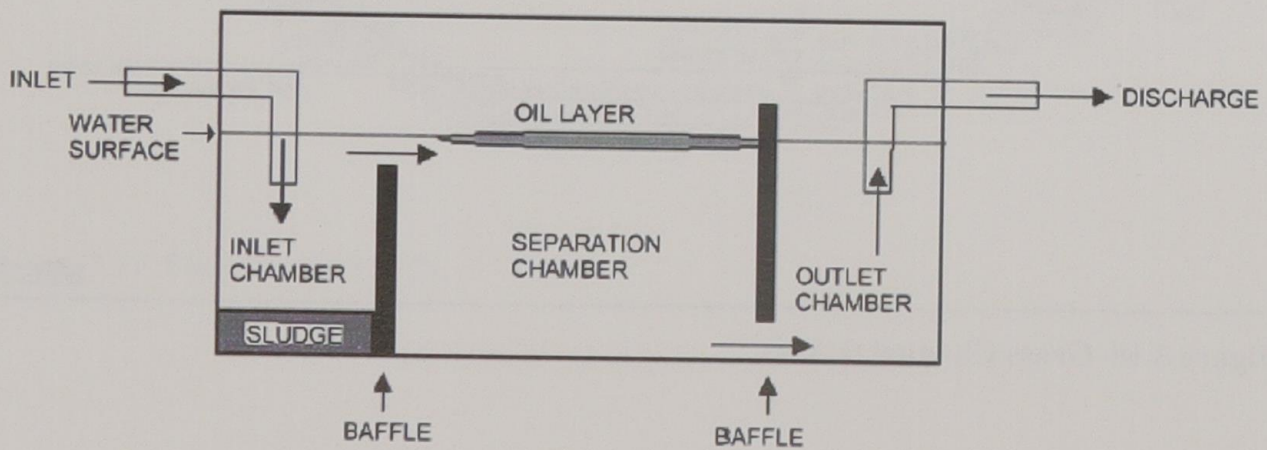
Figure 3.20 Oil and Grit Separator (LA-6)
