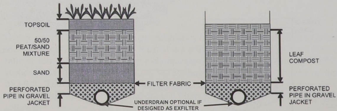
TYPICAL SECTIONS
