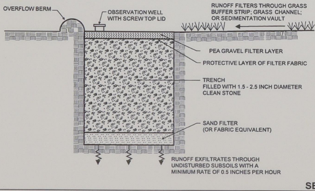
Figure 3.8 Infiltration Trench/Chamber (I-1)
