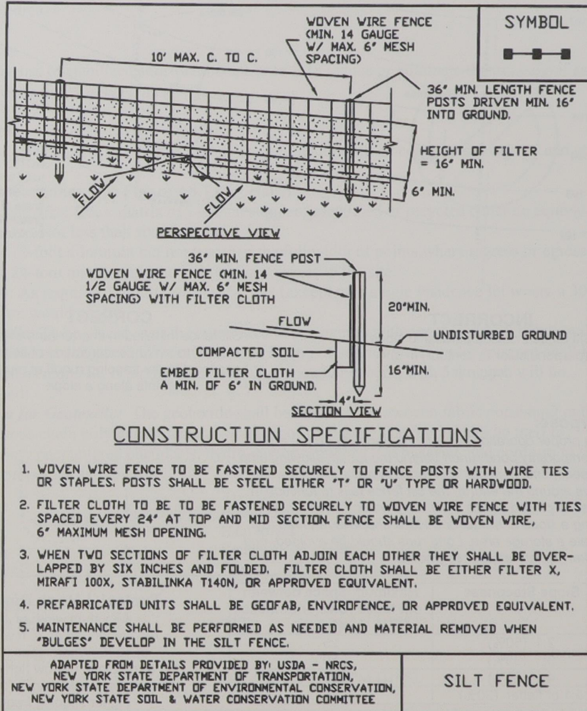
Figure A7.1 Silt Fence
