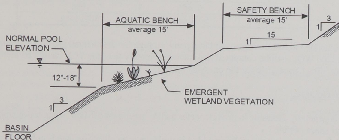
Figure 3.4. Typical Stormwater Pond Geometry Criteria From the Georgia Stormwater Management Manual (ARC, 2001)
