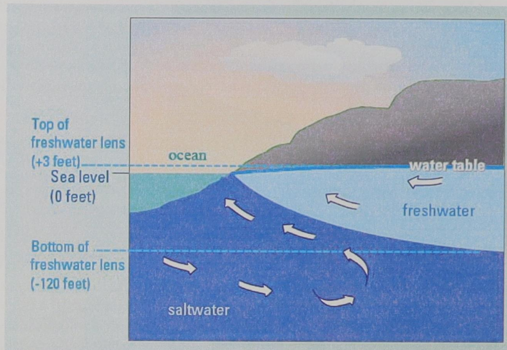
Figure 1.10 Idealized Ghyben-Herzberg lens vs. Reality: transition zone between fresh water and saltwater results in considerably less “useable” fresh water lens thickness than predicted by the 1:40 relationship. (USGS 2008, Gordon Tribble)
