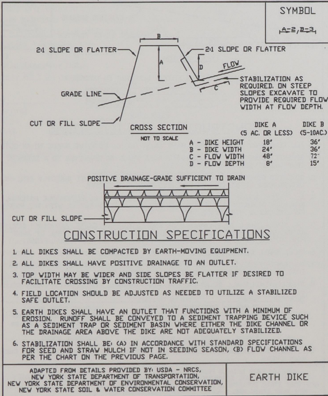
Figure A2.2 Earth Dike
