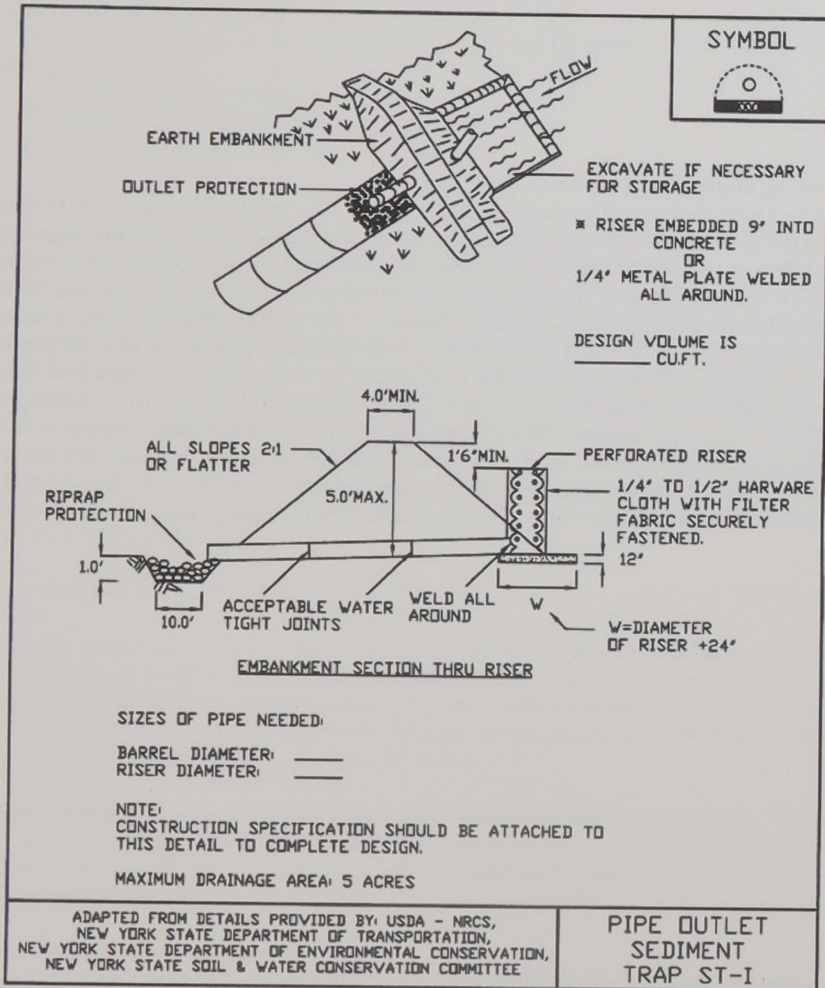
Figure A6.1 Pipe Outlet Sediment Trap
