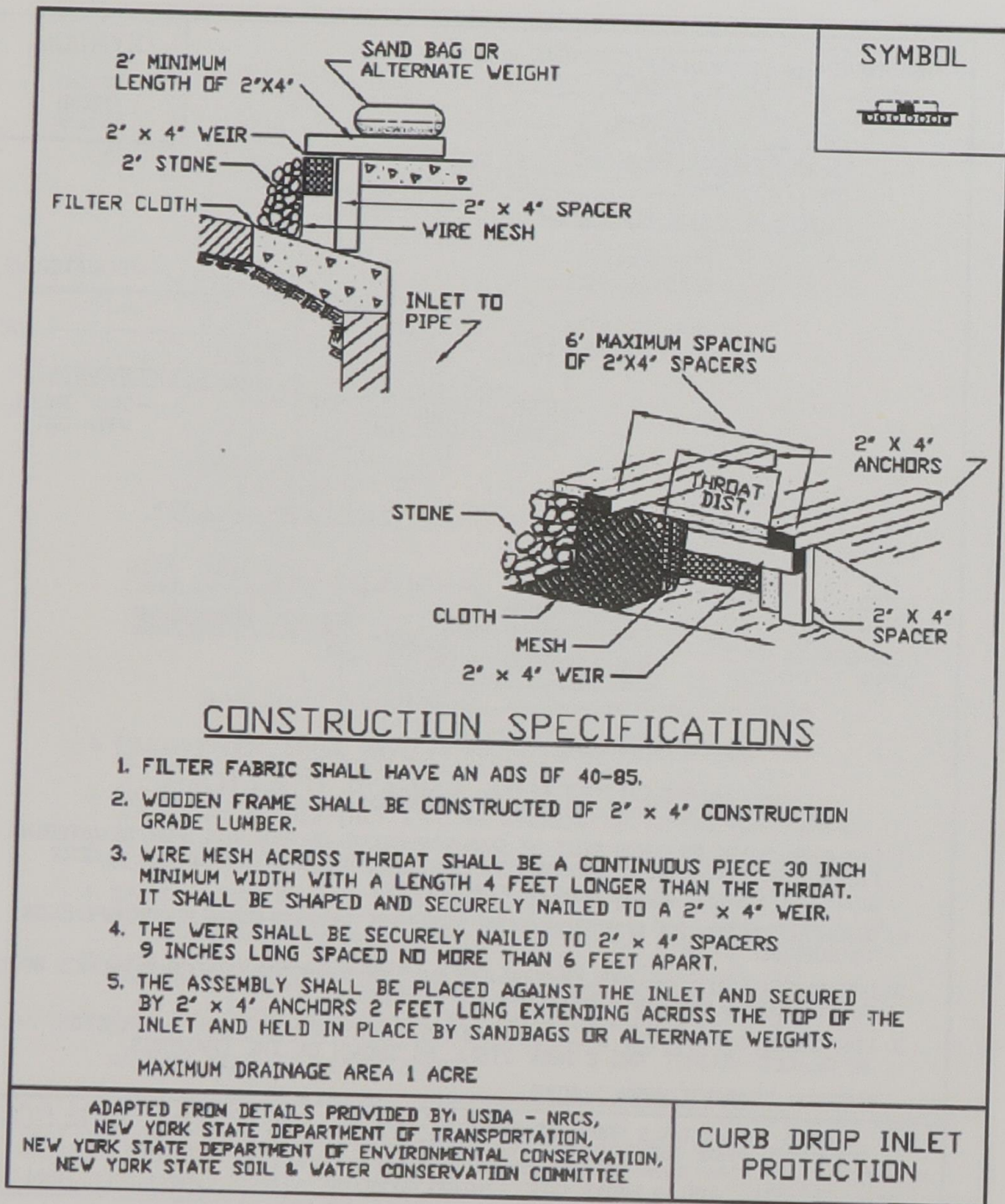
Figure A9.4 Curb Drop Inlet Protection
