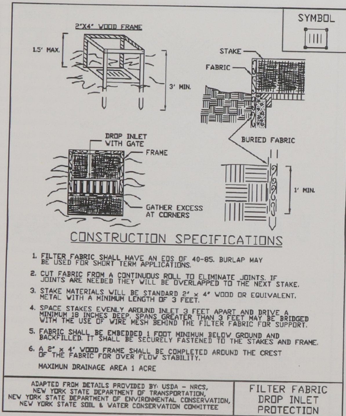
Figure A9.2 Filter Fabric Drop Inlet Protection
