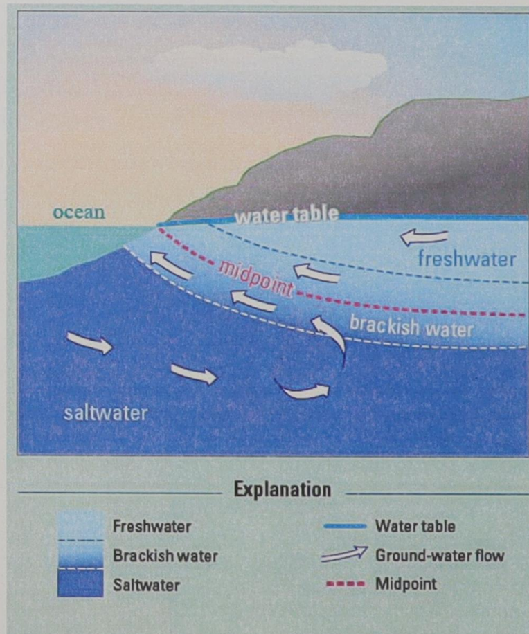
Figure 1.10 Idealized Ghyben-Herzberg lens vs. Reality: transition zone between fresh water and saltwater results in considerably less “useable” fresh water lens thickness than predicted by the 1:40 relationship. (USGS 2008, Gordon Tribble)
