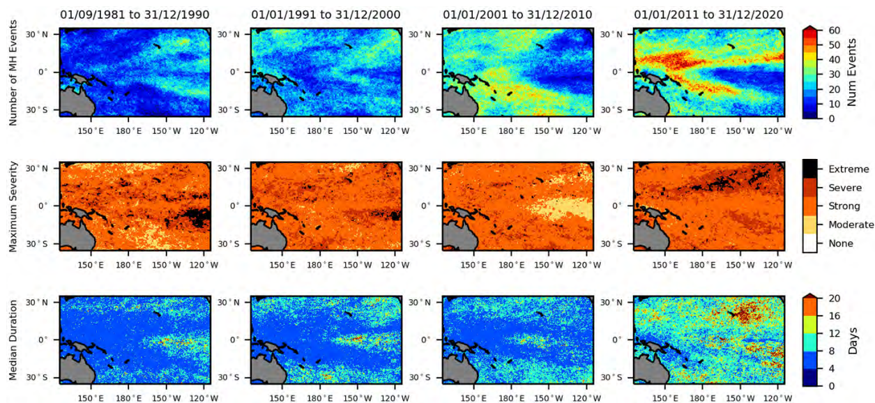
Figure 21. Marine Heat Wave Summaries. Daily NOAA OISSTv2.1 SST data 6 for 1981–2020 were used to calculate number of marine heat wave (MH) events (top row), maximum severity 9 (middle row) and median duration (bottom row). The climatology period was set from 1981–2010 for calculation of the 90th percentile threshold. Summaries are split into decadal periods from left to right: 1980s, 1990s, 2000s, 2010s.
