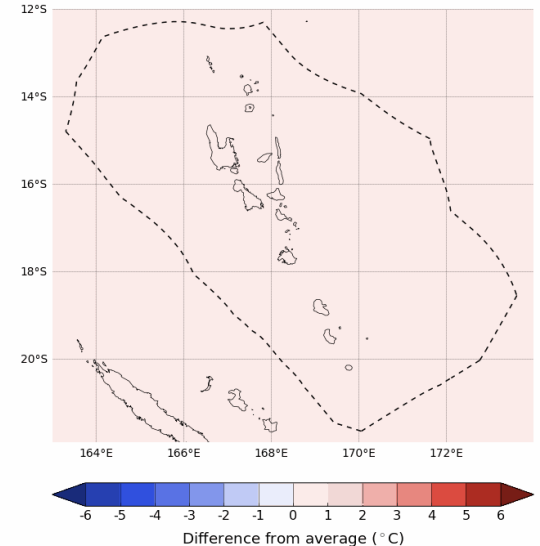
Difference from average mean minimum temperature forecast for May 2023
