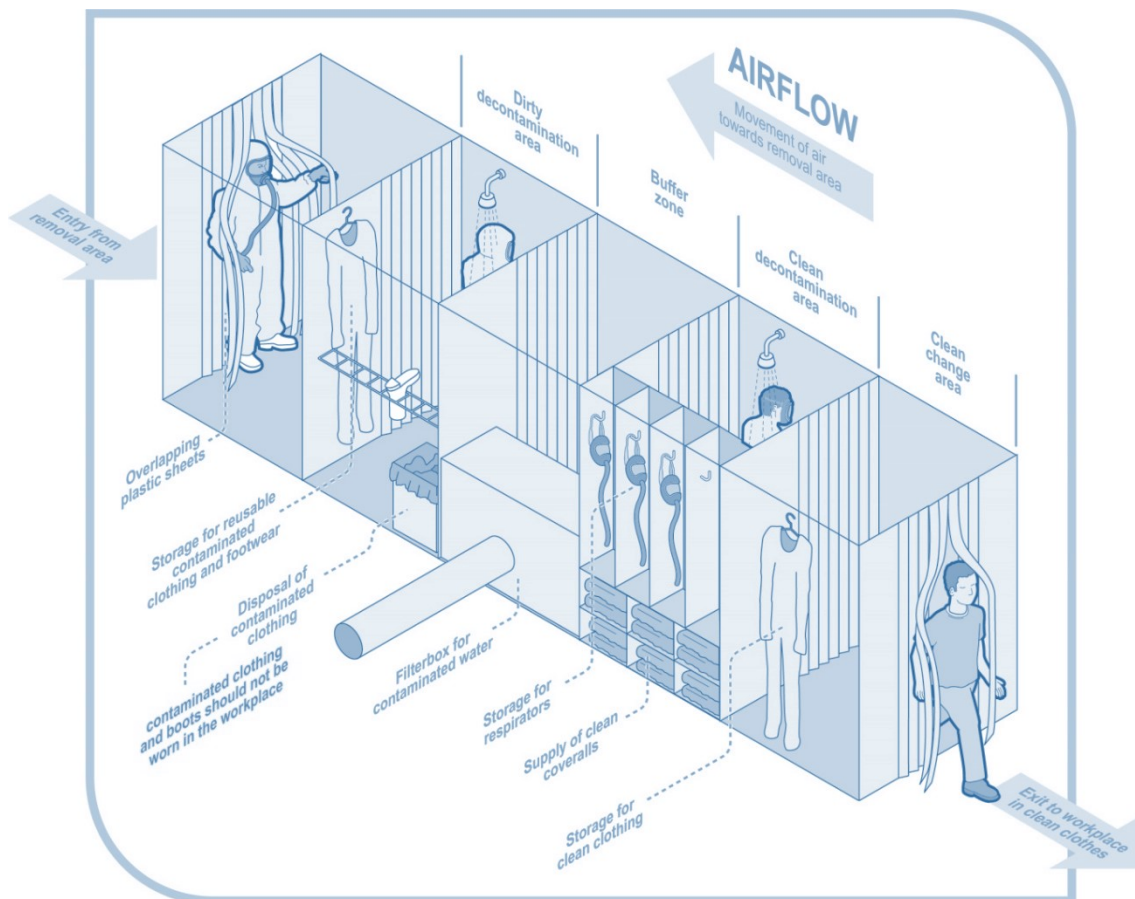
Figure 7: Decontamination unit. Source: https://www.worksafe.govt.nz/dmsdocument/8-acop-management-and-removal-of-asbestos
