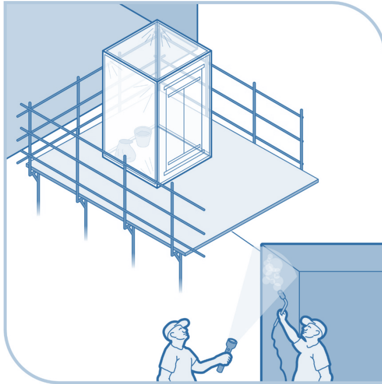
Figure 9: Building and using a mini enclosure. Source: https://www.worksafe.govt.nz/dmsdocument/8-acop-management-and-removal-of-asbestos
