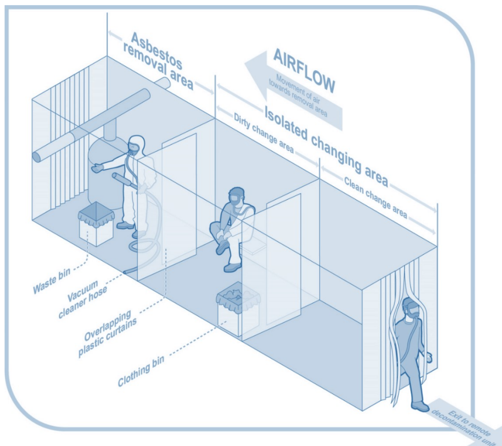
Figure 8: Preliminary decontamination procedure where a remote decontamination unit is used. Source: https://www.worksafe.govt.nz/dmsdocument/8-acop-management-and-removal-of-asbestos
