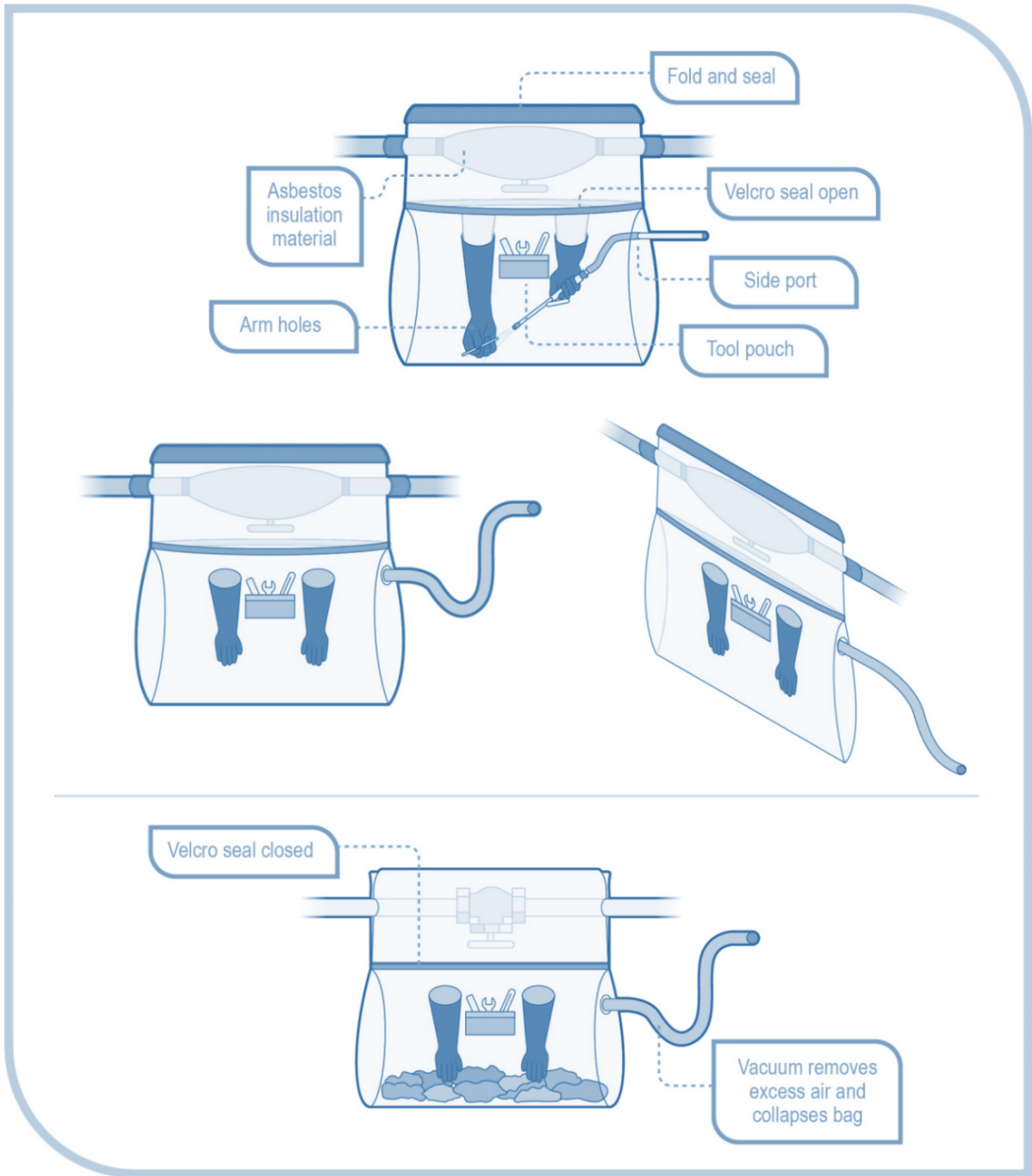
Figure 10 Using a glove bag. Source: https://www.worksafe.govt.nz/dmsdocument/8-acop-management-and-removal-of-asbestos
