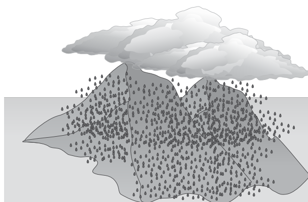
Figure 3.3 Rainfall is higher in mountainous areas. On larger islands (such as Viti Levu and Vanua Levu), rainfall is also greater on the windward (south-east) sides.
