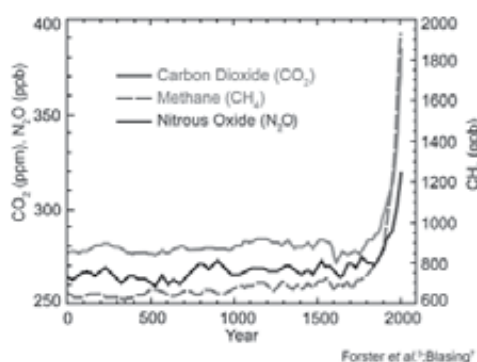
Increases in concentrations of these gases since 1750 are due to human activities in the industrial era. Concentration units are parts per million (ppm) or parts per billion (ppb), indicating the number of molecules of the greenhouse gas per million or billion molecules of air.
