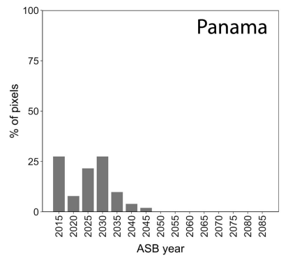
South-East Pacific. Histograms of the distribution of projected timing among reef pixels of the onset of annual severe bleaching (ASB) conditions under SSP5-8.5.
