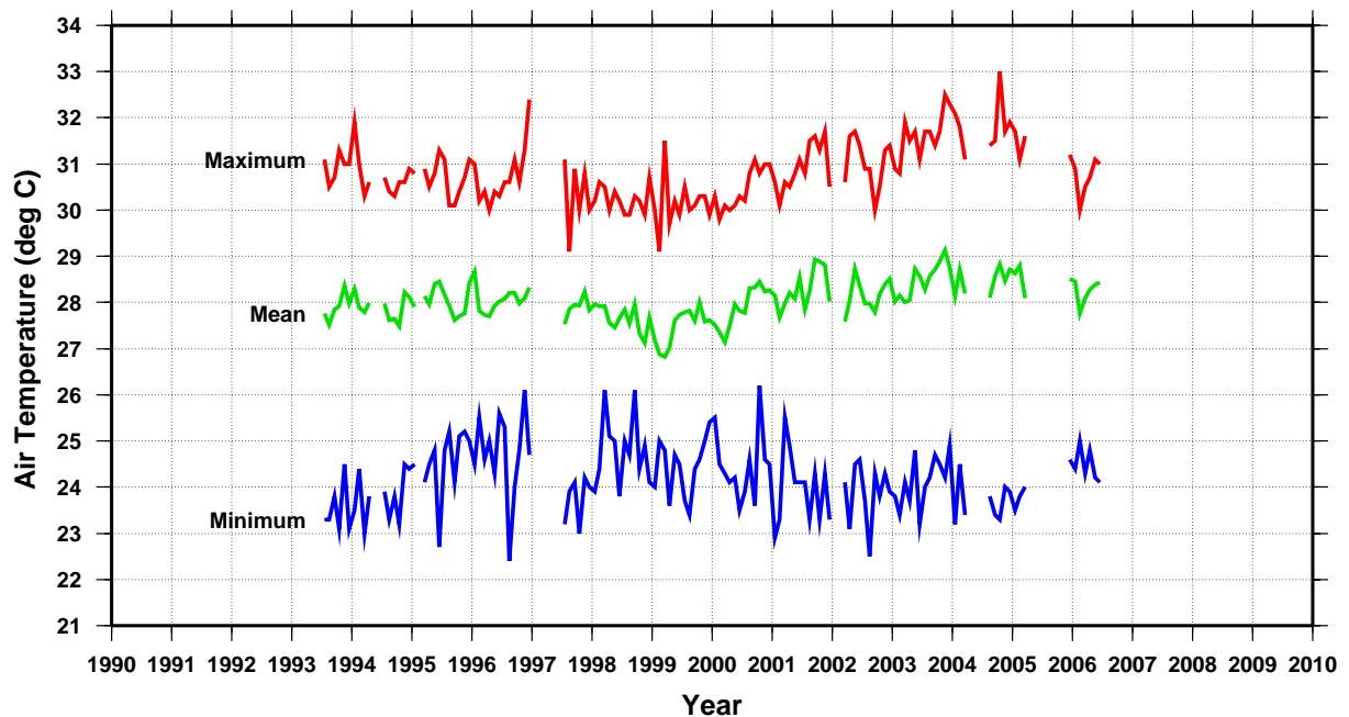
Monthly air temperature at Nauru SEAFRAME gauge
