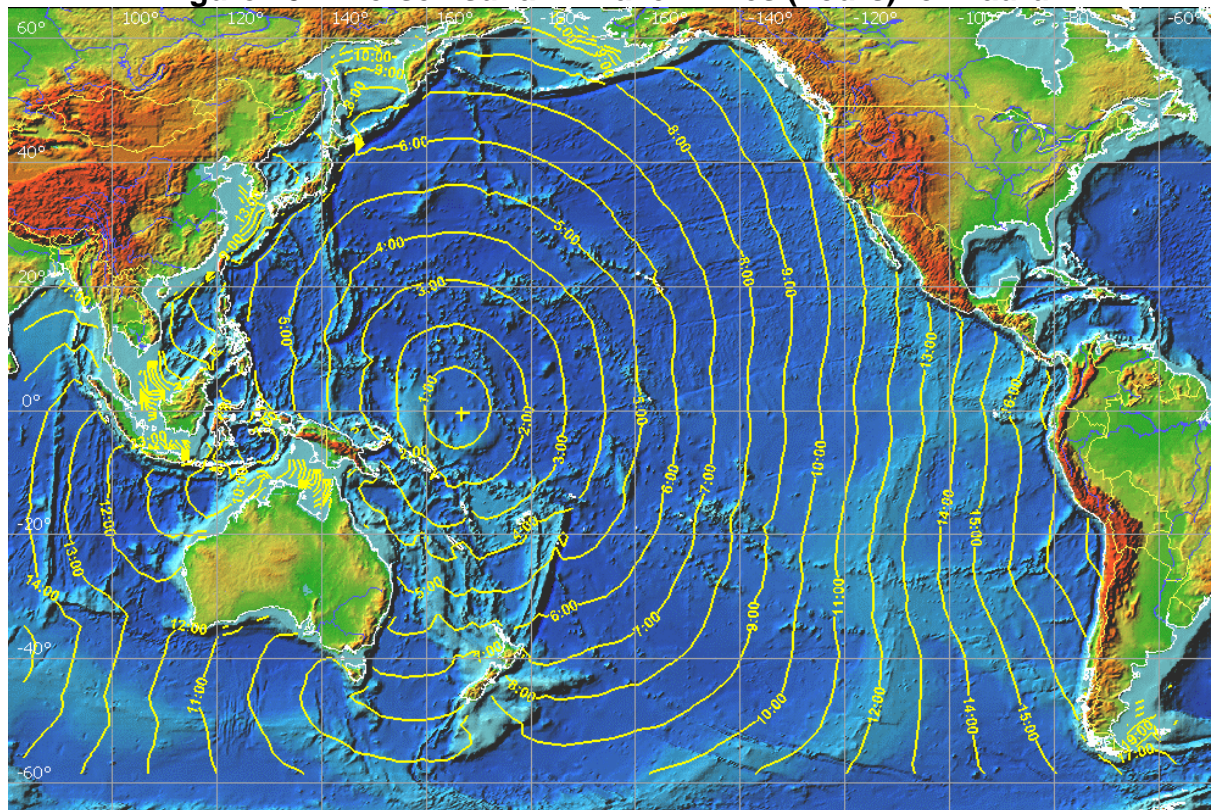
Figure 10. Inverse Tsunami Travel Times (hours) for Nauru.
