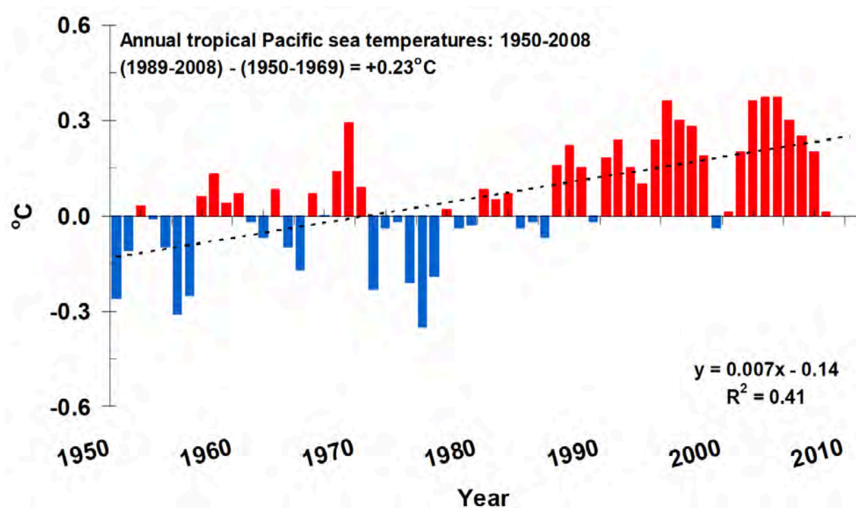
Figure 9: Annual tropical Pacific sea temperatures: 1950–2007
